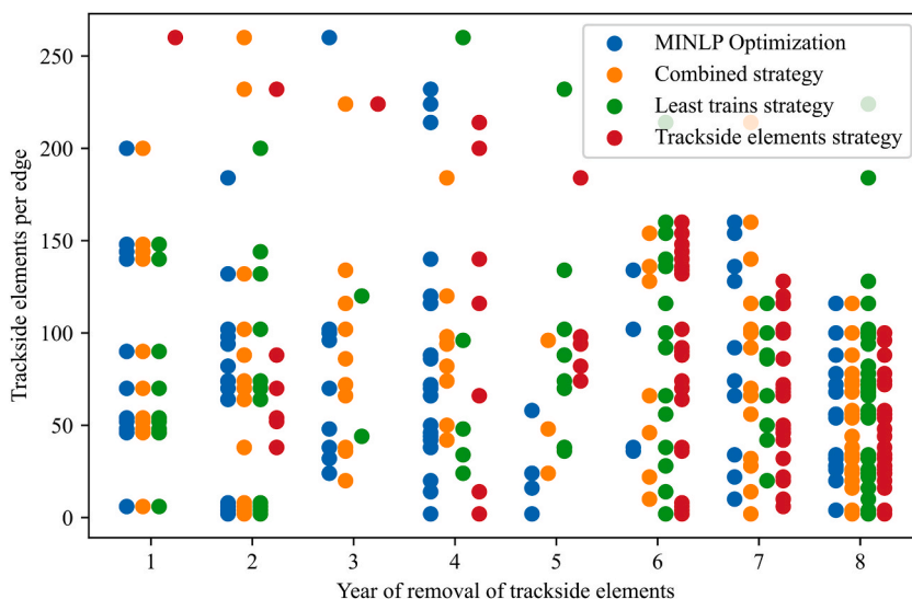
Fig. 5. Trackside elements removal moment (year).
