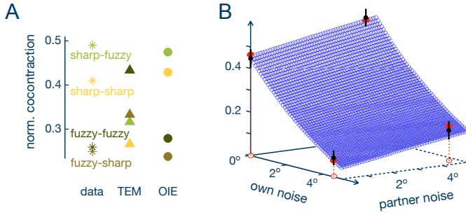
Fig. 4. Results of computational modeling the coactivation adaptation to own and partner noise. (A) Comparison of coactivation observed during the experiment and predicted by the two models described in the text. The TEM model cannot catch the modulation of coactivation with different noise conditions observed in the data while the OIE model predicts well their trend. (B) The OIE model predicts a decrease of coactivation with own noise and an increase with partner noise.
