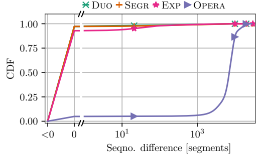
Fig. 7. Difference between received and expected segment sequence number.
