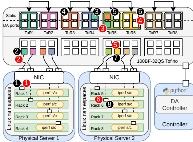
Fig. 16. Illustration of an 8 ToR testbed setup.
