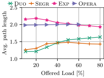
Fig. 8. Comparison of the traffic weighted average path length.
