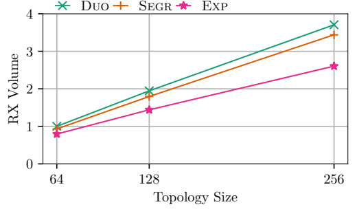
Fig. 14. Impact of topology size on RX volume.
