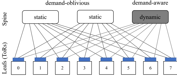
Fig. 1. TMT network example with eight ToR switches and three spine switches from which two are static matchings and one is a dynamic matching. Each spine switch has eight input and output ports.
