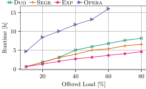
Fig. 13. Comparison of simulation wall clock time.
