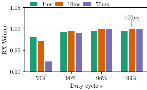
Fig. 11. Impact of period \rho and duty cycle on RX volume. Load is 40%.
