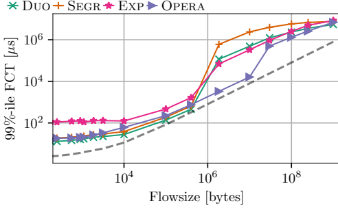
Fig. 6. Comparison of 99%-ile FCT by flow size.
