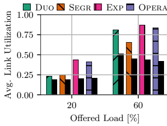
Fig. 9. Comparison of the average link utilization.
