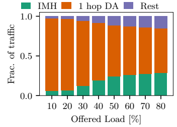
Fig. 10. Comparison of Duo paths' characteristics: IMH vs. 1-hop DA.
