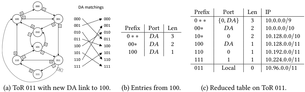
Fig. 4. The new forwarding tables of ToR 011 after the establishment of the DA-link from 011 to 100.
