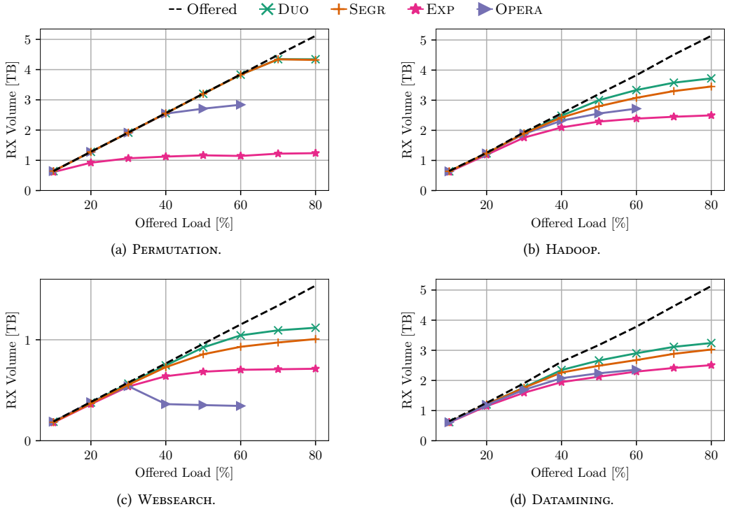
Fig. 5. Total received volume within 10s against total offered load. DUO outperforms the baselines SEGR, EXP, and OPERA.
