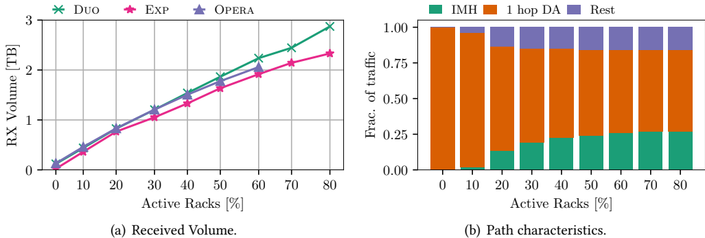
Fig. 15. RX volume and fraction of traffic forwarded via IMH paths for skewed connectivity patterns.
