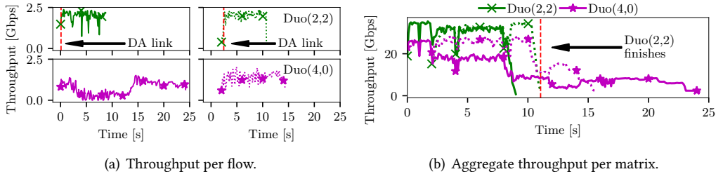
Fig. 17. Throughput over time.
