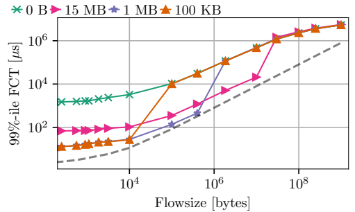
Fig. 12. Impact of small flow threshold on FCTs by flow volume.
