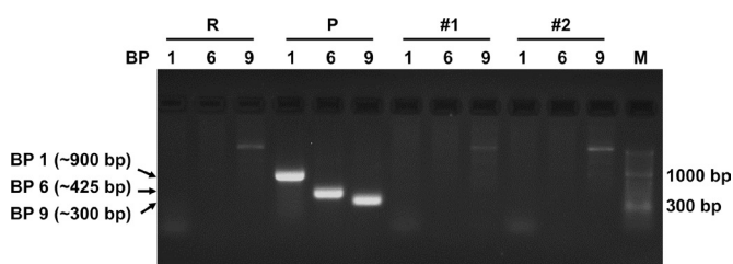
Figure 4 Segregation of the genomic rearrangement in the patient's offspring. PCR was performed on genomic DNA samples to amplify breakpoints 1, 6 and 9 shown in figure 1A. R=reference (unaffected individual), p=patient, #1, 2=progeny.
