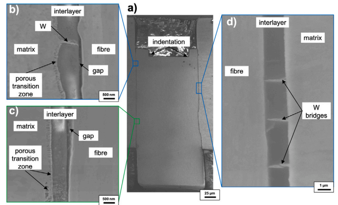
Fig. 8. Cross section of a push-out specimen with Y 2 O 3 (L: 300 μm, F deb : 68.3 N) (a) SEM overview image, (b)–(d) detailed view of interlayer. The debonding for this specimen took place on the fibre surface and the Y 2 O 3 layer is undamaged.
