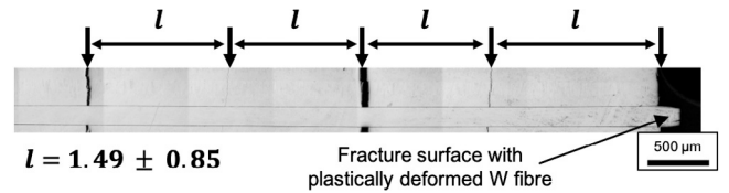
Fig. 17. Multiple matrix failures of W_f/W_{\text{Er}_2\text{O}_3} -TS1 after the tensile test. The distance l of the cracks is approximately constant.
