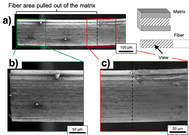
Fig. 15. Fibre which was pulled out of a specimen with \text{Y}_2\text{O}_3 interlayer (L: 591 \mu\text{m} , F_{deb} : 44.3 N) (a) SEM overview of the fibre (b), (c) SEM detailed view of the fibre. No \text{Y}_2\text{O}_3 was visible in the fibre which was pulled out of the matrix. This indicates in combination with the findings from Fig. 14 indicates that \text{Y}_2\text{O}_3 failed on the fibre surface and it was stuck to the matrix.
