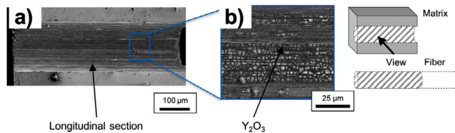
Fig. 14. Cross-section of the matrix of a pull-out sample with a \text{Y}_2\text{O}_3 interlayer after the test (L: 591 \mu\text{m} , F_{deb} : 44.3 N) (a) SEM overview image (b) SEM detail image of the interlayer region. Over the entire matrix where the fibre was pulled out a rough structured layer of \text{Y}_2\text{O}_3 is visible.
