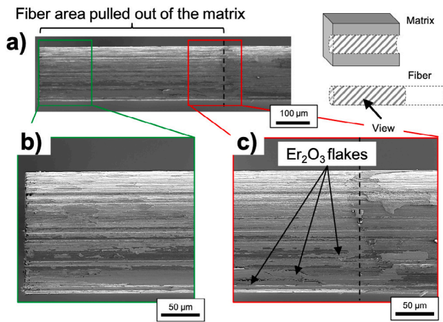
Fig. 13. Fibre which was pulled out of a specimen with \text{Er}_2\text{O}_3 interlayer (L: 583 \mu\text{m} , F_{deb} : 37.7 N) (a) SEM overview of the fibre (b), (c) SEM detailed view of the fibre. Some \text{Er}_2\text{O}_3 was visible in the fibre which was pulled out of the matrix. This indicates in combination with the findings from Fig. 12 indicates that \text{Er}_2\text{O}_3 failed within the interlayer.
