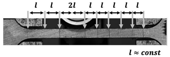
Fig. 16. Multiple matrix cracks of W_f/W_{\text{Y}_2\text{O}_3} -TS6 during the tensile test. The distance l of the cracks is approximately constant.
