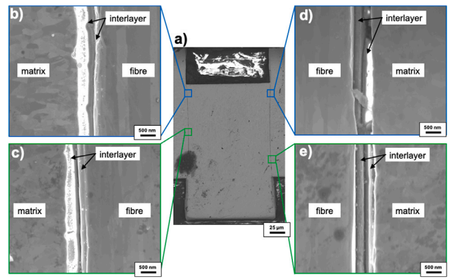
Fig. 7. Cross section of a push-out specimen with Er 2 O 3 interlayer (L: 232 μm, F deb : 42.8 N) (a) SEM overview image, (b)–(e) detailed view of interlayer. The debonding for this specimen took place within the Er 2 O 3 layer. (The different appearance of the two interlayer parts is related to charging caused by epoxy impurities on the interlayer surface).
