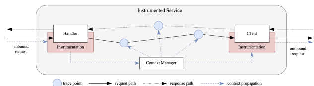
Figure 1: Context propagation in an instrumented service (inspired by Shkuro [26])
