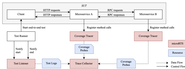
Figure 2: Overview of the microRTS test tracing architecture
