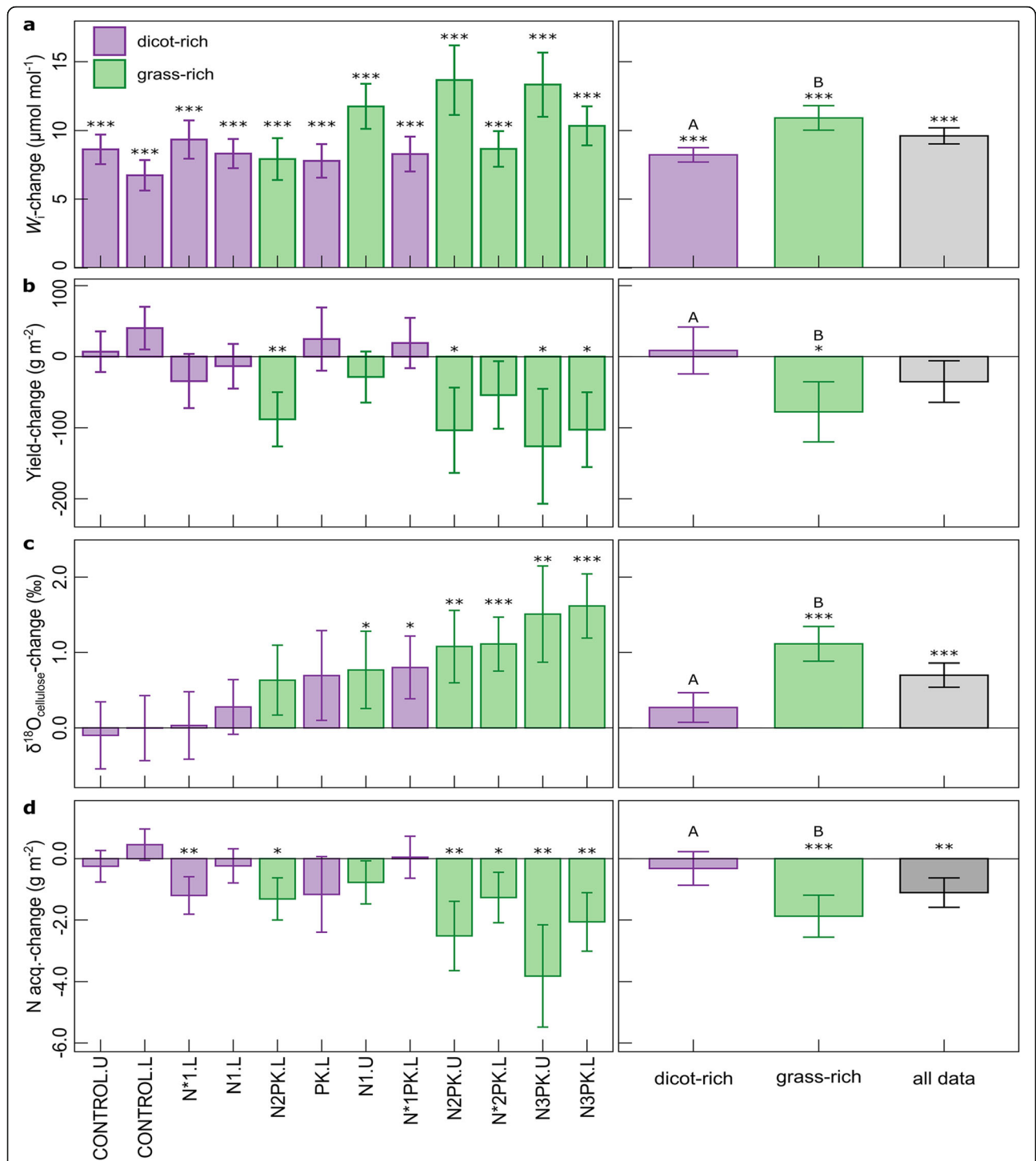
Fig. 3 Long-term changes in physiological parameters at the Park Grass Experiment. Intrinsic water-use efficiency-change ( W_f -change) (a), hay yield-change (b), \delta^{18}\text{O}_{\text{cellulose}} -change (c), and nitrogen acquisition-change (d) during the last century. Changes were calculated as the difference between period 2 (2004–2018) and period 1 (1917–1931). Results are presented for each fertilizer treatment (in the order of the treatment effect on the long-term \delta^{18}\text{O}_{\text{cellulose}} -change), the mean of all dicot-rich and grass-rich treatments, and all treatments combined. Bar plots and error bars represent the calculated difference \pm SE (SE calculated as SE from period 1 + SE from period 2; n = 11\text{--}15 in each period for each treatment depending on data availability; see Additional file 1: Table S1 for details). t tests were used for determining if the long-term changes were statistically significant and significance is presented when P < 0.05 . Significance levels: * P < 0.05 ; ** P < 0.01 ; *** P < 0.001 . Significant differences between grass-rich and dicot-rich treatments are designated with different capital letters
