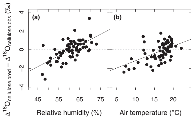
Fig. 3 Difference between predicted and observed \Delta^{18}O_{cellulose} (a) in relation to relative humidity (RH), when \Delta^{18}O_{cellulose} was predicted with a constant p_{ex}p_x = 0.556 and a temperature-dependent \epsilon_{bio} (as in the ‘standard simulation’), and (b) in relation to air temperature, when \Delta^{18}O_{cellulose} was modelled using a constant \epsilon_{bio} = 27\text{‰} and a RH-dependent p_{ex}p_x (as in the ‘standard simulation’). RH and air temperature represent the 400 GDD average of midday ( \pm 3 h around noon) humidity and daily mean temperature, respectively.
