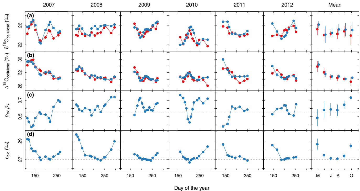
Fig. 5 Time course (a) of the oxygen isotope composition of leaf cellulose ( \delta^{18}\text{O}_{\text{cellulose}} ) and (b) of the isotopic enrichment of cellulose relative to source water ( \Delta^{18}\text{O}_{\text{cellulose}} ). Red dots, observed data; blue dots, model predictions obtained with the 'standard parameterization' with temperature-dependent \epsilon_{\text{bio}} and RH-dependent p_{\text{ex}}p_x . Observed \Delta^{18}\text{O}_{\text{cellulose}} was calculated from the \delta^{18}\text{O}_{\text{cellulose}} of the sample and average observed \delta^{18}\text{O}_{\text{source}} during 400 GDD before the sampling date (see Eqn S10 in Supporting Information Methods S2). (c) Time course of p_{\text{ex}}p_x as estimated from midday relative humidity and averaged over the integration time (400 GDD). The horizontal dashed line indicates the value for p_{\text{ex}}p_x used in the constant- p_{\text{ex}}p_x simulations ( p_{\text{ex}}p_x = 0.556 ). (d) Calculated average \epsilon_{\text{bio}} for the total substrate used in cellulose synthesis of a given leaf sample throughout the 400 GDD integration time. The horizontal dashed line shows \epsilon_{\text{bio}} = 27\text{‰} . Average (2007–2012) monthly values of \Delta^{18}\text{O}_{\text{cellulose}} , \delta^{18}\text{O}_{\text{cellulose}} , p_{\text{ex}}p_x and \epsilon_{\text{bio}} are displayed on the right-hand side, with error bars denoting the standard deviations. Linear regression analysis indicated a significant trend for monthly mean \Delta^{18}\text{O}_{\text{cellulose}} (observed \Delta^{18}\text{O}_{\text{cellulose}} = 37.28 - 0.83 \text{ month} ; R^2 = 0.90 ; P < 0.01 ; predicted \Delta^{18}\text{O}_{\text{cellulose}} = 36.59 - 0.69 \text{ month} ; R^2 = 0.68 ; P < 0.05 ) and monthly mean p_{\text{ex}}p_x ( p_{\text{ex}}p_x = 0.30 + 0.04 \text{ month} ; R^2 = 0.85 ; P < 0.01 ).
