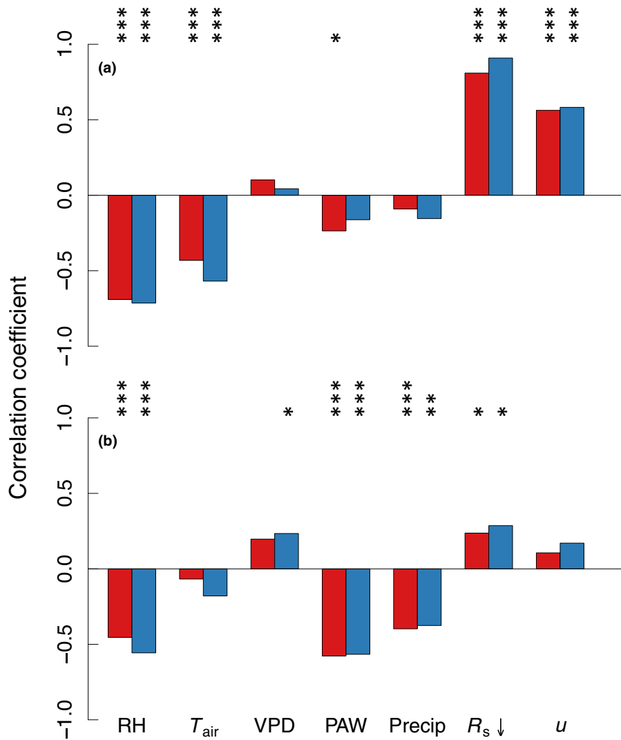
Fig. 6 Correlation coefficients for the relationships between (a) \Delta^{18}\text{O}_{\text{cellulose}} and meteorological variables and (b) \delta^{18}\text{O}_{\text{cellulose}} and meteorological variables: relative humidity (RH), air temperature ( T_{\text{air}} ), vapour pressure deficit of the air (VPD), plant-available water (PAW), precipitation amount (Precip), incoming (downward) short-wave radiation ( R_s \downarrow ) and wind speed ( u ). Red bars, observed data; blue bars, predicted data. RH, VPD and u represent midday ( \pm 3 h around noon) values averaged over the integration time \Delta t (400 GDD); T_{\text{air}} represents daily mean values averaged over \Delta t ; and R_s \downarrow and Precip represent the total sums of incoming short-wave radiation and the total precipitation within \Delta t . All predictions were made with the model in 'standard parameterization', including temperature-sensitive \epsilon_{\text{bio}} and relative humidity-sensitive p_{\text{ex}p_x} . Asterisks indicate the significance levels: ***, P < 0.001 ; **, P < 0.01 ; *, P < 0.05 .
