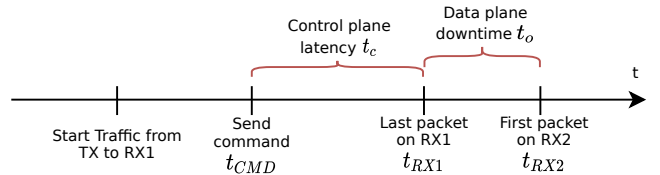
Fig. 4. Idealized timeline of the measurement. Characteristic duration of reconfiguration (red braces). RX1 and RX2 are the ports between the circuit is changed.
