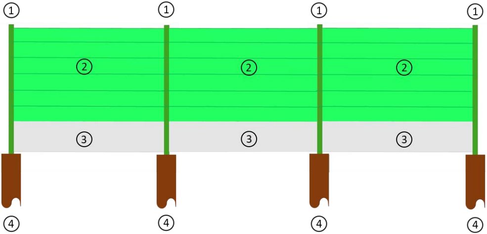
FIG. 13: Design of a noise barrier
