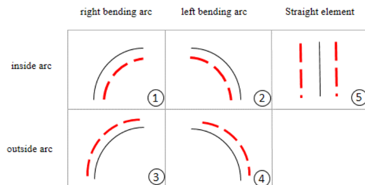
FIG. 18: Relation of noise barrier (red, broken line) to arc element (black, continuous line)
