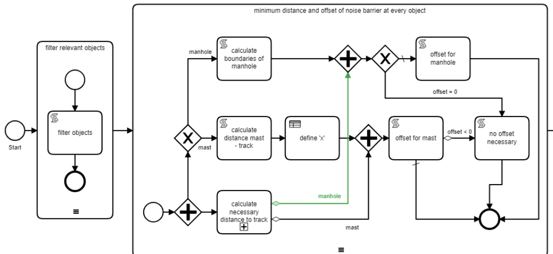
FIG. 21: BPMN diagram for the design of by-passes part I: Filter relevant objects, minimum distance and offset of noise barrier at every object
