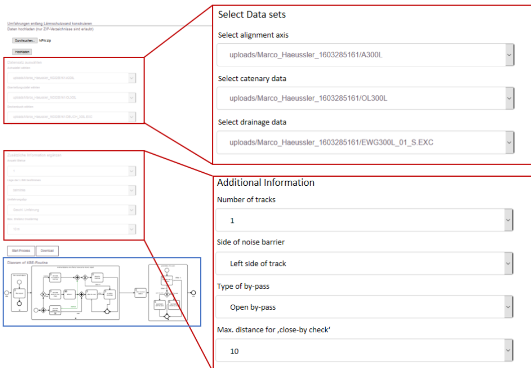
FIG. 23: Web-based user interface for choosing the data to submit to the KBE system (server-side) and setting additional user inputs via dropdowns (red). The BPNM process diagram is also displayed to the user (blue).
