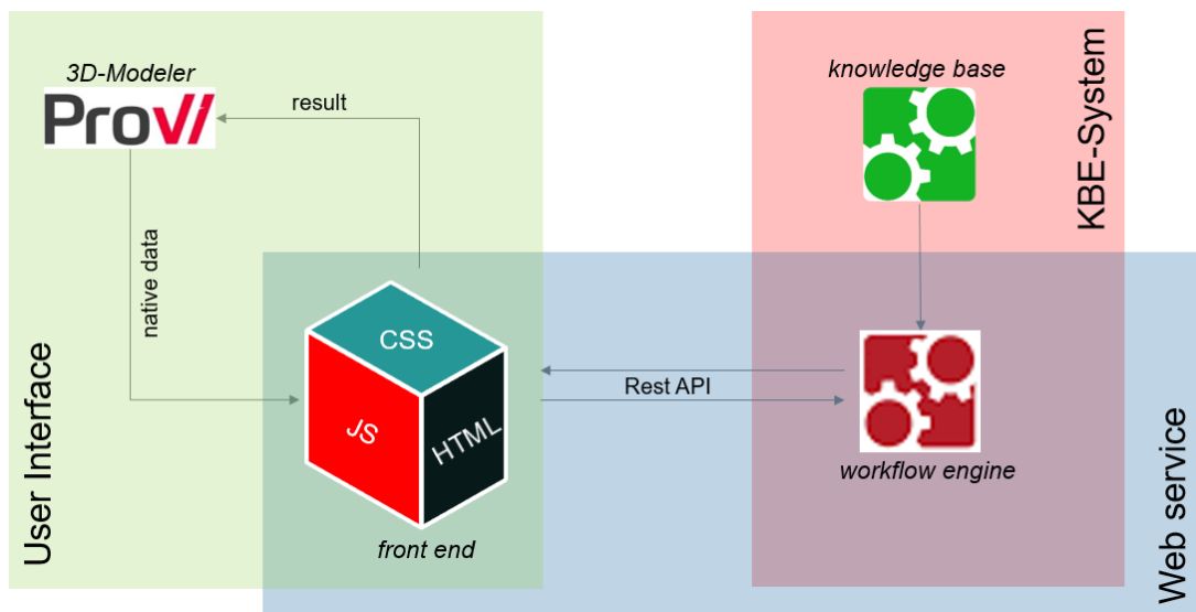
FIG. 12: Software configuration
