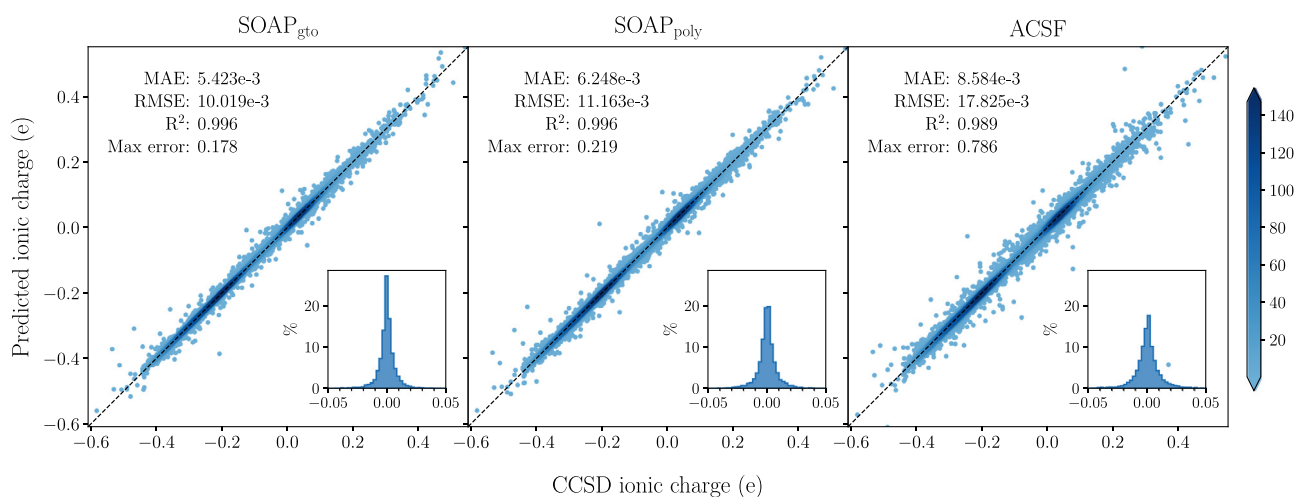
Fig. 10. Parity plot of ionic charge prediction results from the test set against true CCSD ionic charges. The predictions are performed with kernel ridge regression using SOAP gto (gaussian type orbital basis), SOAP poly (polynomial basis) and ACSF. The mean absolute error (MAE), root mean square error (RMSE), squared Pearson correlation coefficient ( R^2 ) and maximum error are also shown together with the total error distribution in the inset.
