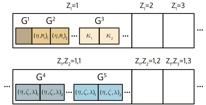
Fig. 4. Structure of the ACSF output vector. The values of the two-body symmetry functions G^1 , G^2 and G^3 are given first for each chemical species present in the dataset. Next the values of the three-body symmetry functions G^4 and G^5 are listed for each unique combination of two chemical species. All symmetry functions except G^1 may also have multiple parameterizations as indicated by the subindices.
