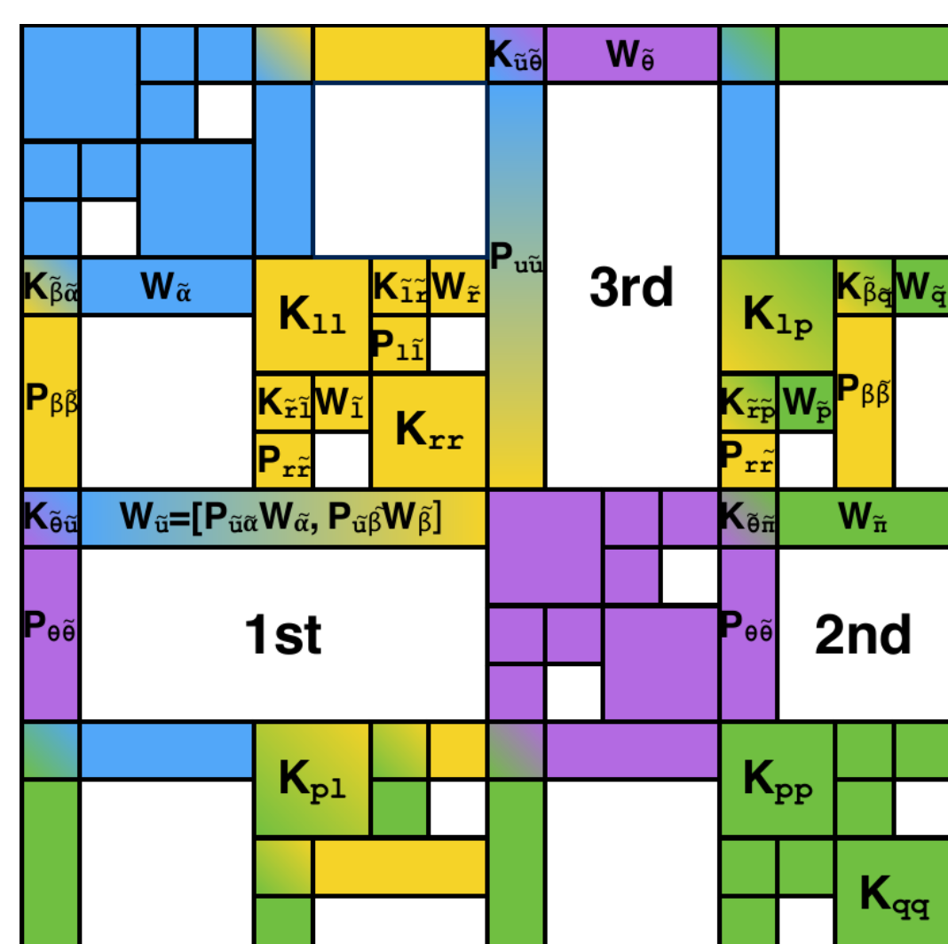
4-process distributed \mathcal{H} -Matrix compression. Mixed colored sections and factors are shared for distributed nodes
