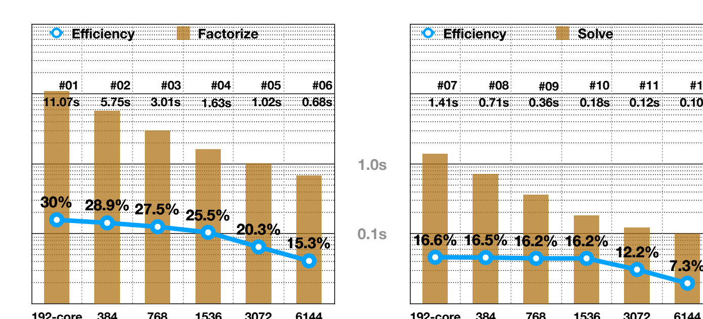
Time for ULV-Factorization (left) and forward-solve (right)
