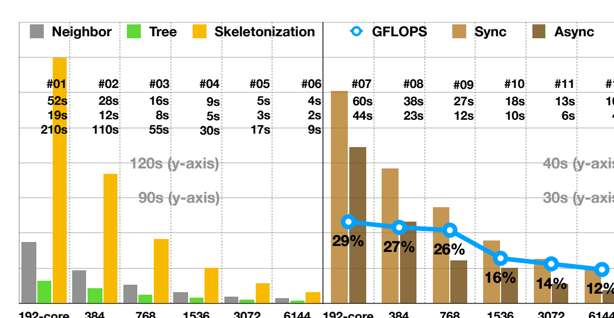
Time for compression (left) and multiplication (right) for a 6-d gaussian kernel matrix of 64M-by-64M
