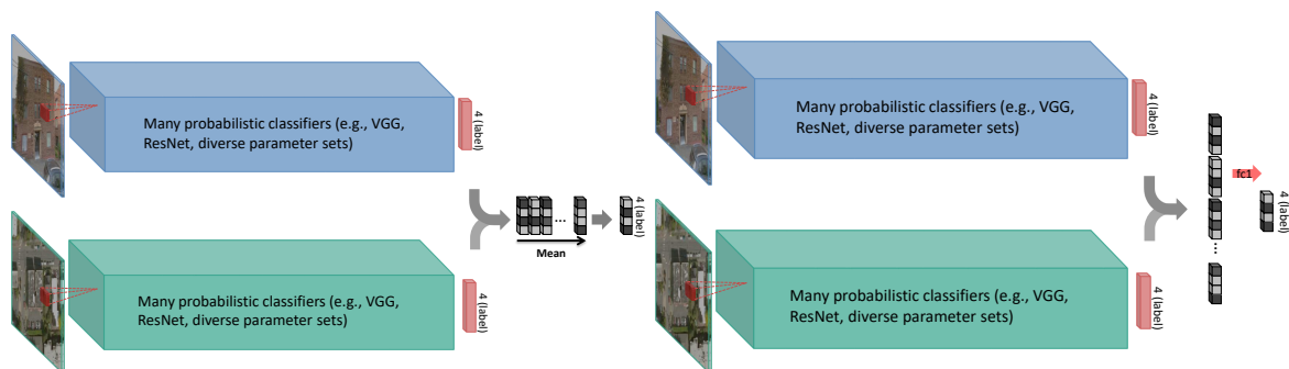
Figure 4. A schematic drawing of the two decision-level fusion strategies—model blending (left) and model stacking (right)—exploited in this article. Model blending takes the mean of the softmax layer of multiple models, while model stacking concatenates those softmax vectors, and connects to a final softmax layer. Both of the fusion strategies act on a decision level, which allows networks for individual data type to be trained independently.
