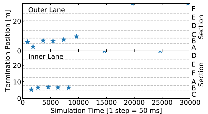
Fig. 16. Scenario 1. Termination position of the robot at each trail is marked by a star. During the first 10,000 simulation steps, the robot triggers resets at each trial in the first turn in both directions. Afterwards, it has successfully learned how to follow the lane, only triggering a reset when a complete lap is finished.
