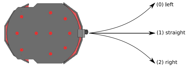
Fig. 5. Action space in lane-keeping task with three discrete actions: (0) Turn left: Set left motor speed to v_s - v_r and right motor speed to v_s + v_r . (1) Go straight: Set left and right motor speed to v_s . (2) Turn right: Set left motor speed to v_s + v_r and right motor speed to v_s - v_r .
