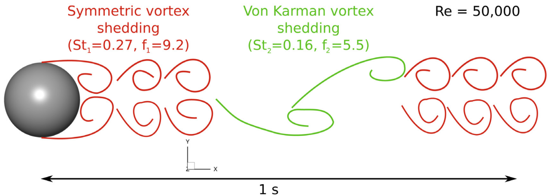
(e) Example of the alternation in time of both shedding types.
