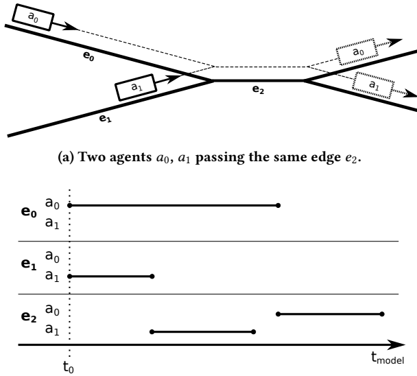
(a) Two agents a_0, a_1 passing the same edge e_2 . (b) Occupancy intervals for edges e_0, e_1, e_2 . Since a_0 and a_1 never share their starting edges with other agents, they can be fast-forwarded across e_0 and e_1 , respectively. Further, since a_0 and a_1 never occupy e_2 at the same time, both can be fast-forwarded across e_2 . Thus, at minimum, the independence intervals of both a_0 and a_1 extend to the time at which the successor edge to e_2 is sensed.
