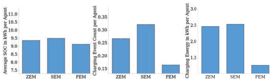
Figure 2: Average SOC, charging event count and charging energy per agent for the three charging behaviours
