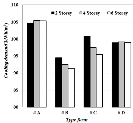
Figure 16. The average cooling loads for building forms during a year in Tabriz.
