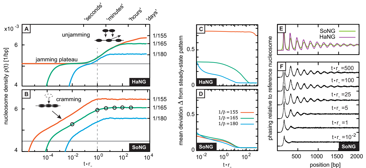
Figure 3. Characterization of nucleosome array assembly within the soft-core model and comparison to hard-core nucleosomes. (A) Time-dependent nucleosome density \rho(t) for the HaNG model (with a logarithmic timescale). Three curves are shown for different final densities, as labeled on the right vertical axis. The gray horizontal line indicates the jamming density at which, statistically, non-overlapping adsorption opportunities have been exhausted. From this point, the hard-core nucleosomes must wait for desorption events to further increase the density (see sketch). The time labels above the figure mark approximate timescales based on the in vitro estimate of (13) (see main text). (B) Same plot for the SoNG model. Soft-core nucleosomes (represented by shaded ellipses in the sketch) have a larger maximal DNA footprint and accordingly have a smaller nominal jamming density (again indicated by a gray line). However, after reaching this density, \rho(t) does not plateau, but instead enters a ‘cramming’ stage. (C) Mean deviation \Delta(t) between the time-dependent nucleosome pattern p(x, t) and its steady-state \bar{p}(x) for the HaNG model (see text for details). The three curves correspond to the same cases as shown in panel (A). (D) Same plot for the SoNG model. (E) Comparison of the equilibrium patterns of the two models at a nucleosome density of 1/(165 \text{ bp}) . (F) Snapshots of the average nucleosome pattern during the filling process of the SoNG model for 1/(165 \text{ bp}) final nucleosome density. The circles on the green line in panel B mark the points in time for which the snapshots are displayed.
