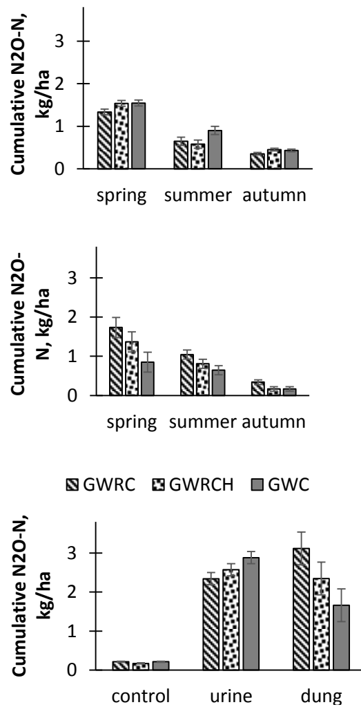
Fig. 2. Cumulative seasonal N 2 O-N emission from urine (top) and dung (middle) and sum of all seasons (bottom)
