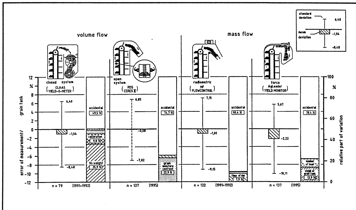
picture 3: Accuracy and error sources of yield measurement systems in combine harvesters
