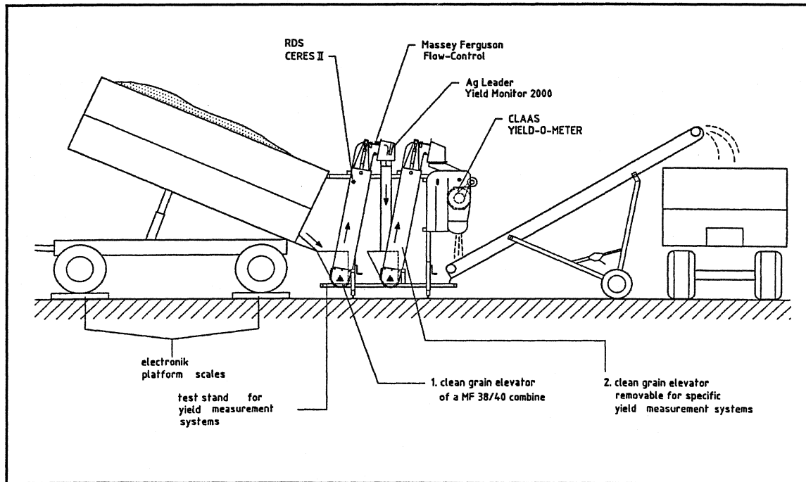
picture 4: Test stand for yield measurement systems in combine harvesters
