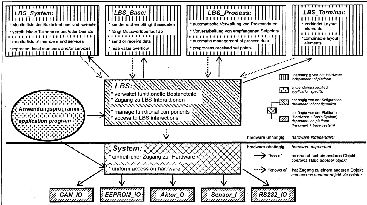
Fig 2: Structure of the library of LBS lib
