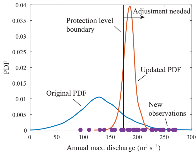
Figure 4. Original and updated PDF based on a period of high new observations of annual maximum discharge. Because the original PDF is so broad, the period of extreme observations results in a strongly shifted updated PDF, the peak of which (corresponding to the estimate of q^{(1)} ) crosses the protection boundary level. Thus, the protection system must be adjusted.
