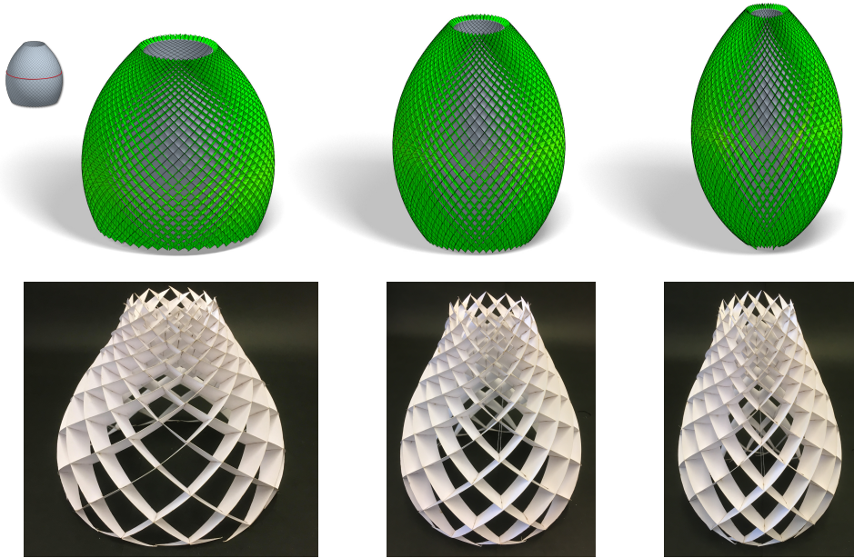
Figure 8: Deformation of the unduloid using the spherical vertex star property. The radius of the red curve was reduced by 10, respectively 20% to drive the deformation. The bottom row shows a corresponding paper model employing a coarser curve network on the upper half of the unduloid.
