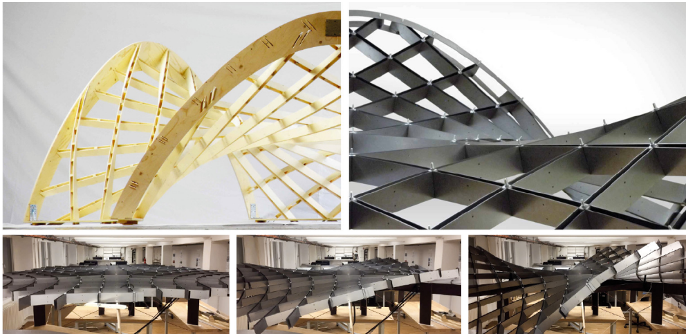
Figure 12: The structure was tested with two prototypes, one in timber and one in steel, each with an approx. 4×4 m span. Left: The lamellas of the timber prototype are arranged on separate levels to allow the use of uninterrupted profiles. Right: The lamellas of the steel prototype are interlocked in one level. They were first assembled flat and then transformed into the curved geometry.
