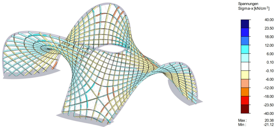
Figure 17: The load-bearing structure of the Asymptotic Gridshell. The lamellas are bent and twisted to form an anticlastic network with two singularities. The diagonal bracing is arranged at every second node. The horizontal supports adjust to the varying inclination angle of the edge beam. The diagram shows the surface stresses of the lamella grid, resulting from both the elastic erection process and self-weight. All stresses stay within the elastic range.
