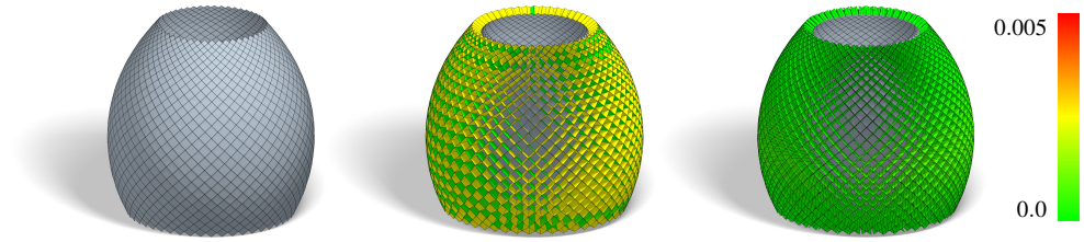
Figure 7: From left to right: Base mesh aligned to curves of constant normal curvature. Initial set of strips, color coded according to developability. Post optimized strips after one round of subdivision and 20 iterations of guided projection.
