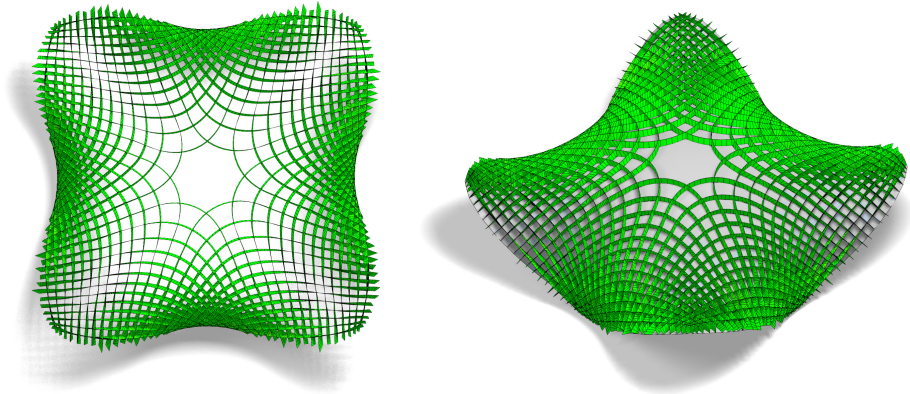
Figure 10: Strips (of radius 1.47) after 2 rounds of subdivision, each followed by 20 iterations of guided projection.
