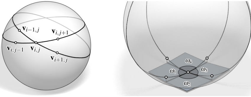
Figure 5: Spherical vertex stars, Meusnier's sphere, and discrete right angle condition \omega_1 + \omega_3 = \omega_2 + \omega_4 .
