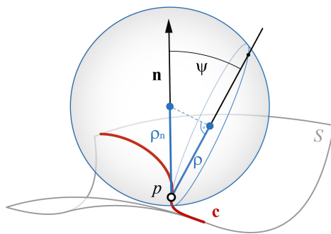
Figure 4: Meusnier's theorem, relating the curvature of a curve \mathbf{c} passing through \mathbf{p} to normal curvature at \mathbf{p} in direction of \mathbf{c}' .
