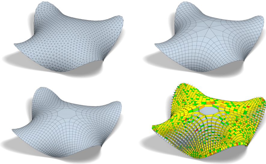
Figure 9: From left to right and top to bottom: Ocean reference surface, isothermic mesh, network of constant normal curvature curves, and the initial set of strips following the curve network.
