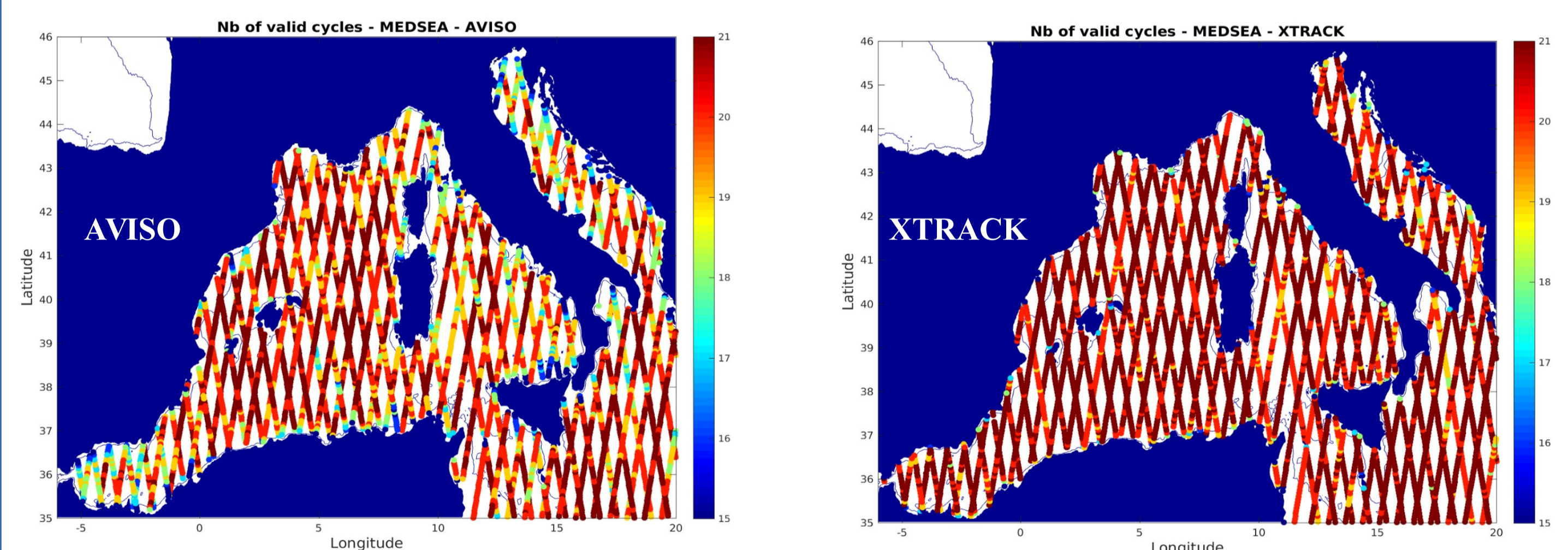
Figure 3: Number of valid cycle for SARAL mission in the West Mediterranean Sea with AVISO and X-TRACK product.
