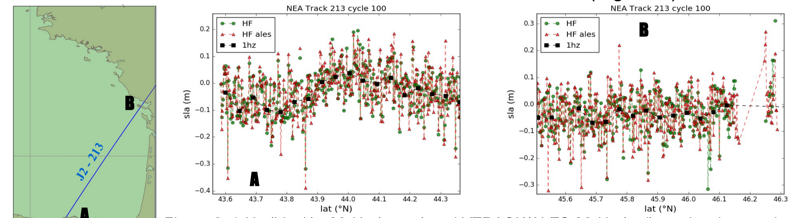
Figure 6: 1-Hz (black), 20-Hz (green) and XTRACK/ALES 20-Hz (red) sea level anomaly along Jason2 track 213 in the Bay of Biscay for the cycle 100
