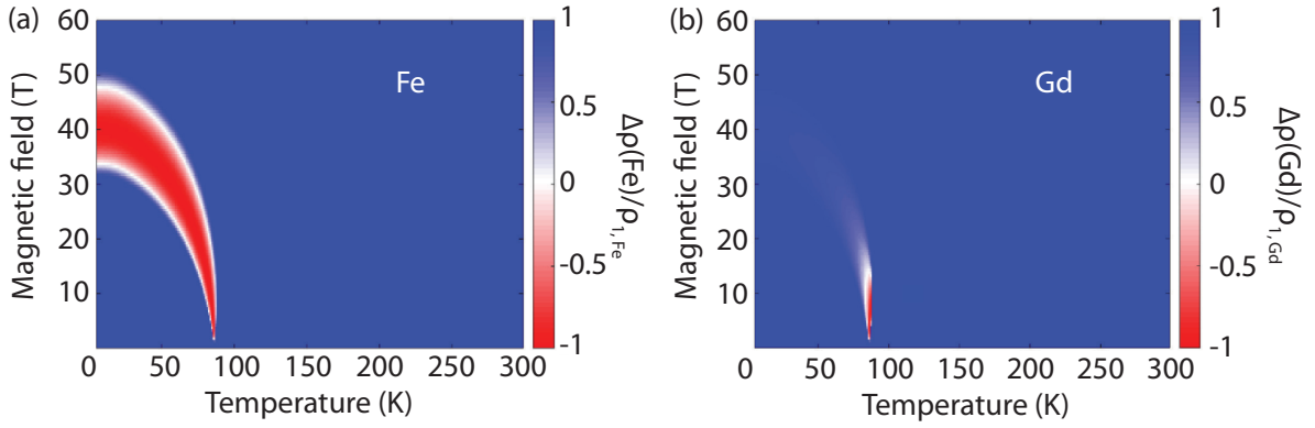
Figure 4.6: Calculation of the expected SMR response in a simplified two sublattice system with a net Fe and a Gd sublattice magnetization. The magnetic properties of this model system are similar to the ones of the InYGdIG sample studied here. The calculations are based on a mean field model and were conducted by R. Schlitz in the course of his master’s thesis at WMI [55]. The sublattice specific (normalized) resistivity modulation amplitude \Delta\rho calculated from the orientation of the sublattice magnetizations \xi_X is depicted as a function of magnetic field and temperature for the net Fe sublattice moments (a) and the Gd moments (b). The red and blue color represent negative and positive \Delta\rho , respectively.
