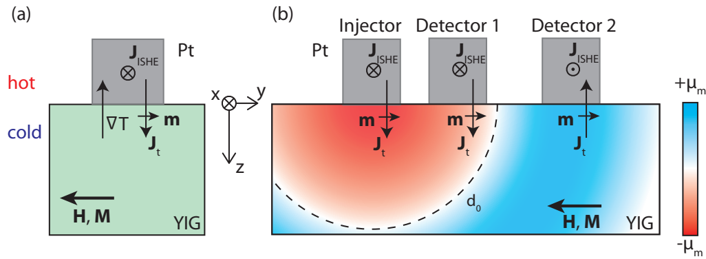
Figure 5.5: (a) Schematic representation of the local (longitudinal) SSE in YIG/Pt. A temperature gradient \nabla T applied across the YIG/Pt interface generates a current \mathbf{J}_t of magnetic moment \mathbf{m} along the temperature gradient into the YIG. The ensuing ISHE current \mathbf{J}_{\text{ISHE}} can be measured in the Pt. (b) Schematic representation of the magnon accumulation profile in YIG where the blue and red color corresponds to a magnon accumulation and depletion (compared to thermal equilibrium), respectively. The sign change of the magnon accumulation occurs at d_0 (black dashed line) and leads to an inversion of the interfacial magnetic moment current \mathbf{J}_t for d > d_0 . Consequently, the measured ISHE voltage is opposite in detector 1 and 2. The white region on the right edge of the YIG film corresponds to thermal equilibrium, where the thermally excited magnon accumulation is relaxed.
