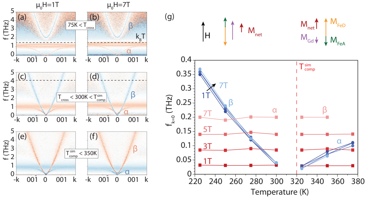
Figure 9.3: Magnon spectrum of GdIG obtained from atomistic simulations, calculated (a)-(b) at T = 75 K, (c)-(d) just below T_{\text{comp}}^{\text{sim}} = 320 K and (e)-(f) above the compensation point. The red and blue color indicates counterclockwise and clockwise precession directions relative to the external magnetic field direction, i.e. positive and negative polarization, respectively. The spectra are calculated for \mu_0 H = 1 T and 7 T revealing the effect of the Zeeman shift of the “+” polarized mode (red). The black dashed line corresponds to the thermal energy k_B T . (g) Temperature and magnetic field dependence of the frequency of the k = 0 magnons for the \alpha and \beta modes. The red and blue colored symbols mark the positive and negative polarization of the magnon branches. The orientation of the sublattice and net magnetization with respect to the external field is depicted by arrows for temperatures above and below the compensation point T_{\text{comp}}^{\text{sim}} . The calculations were conducted by J. Barker and the figures are adapted from Ref. [129].
