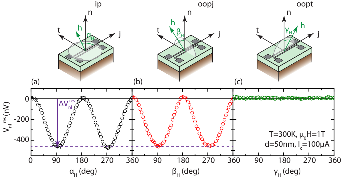
Figure 6.2: Non-local resistive voltage V_{nl}^{\text{res}} in a YIG/Pt bilayer measured at T = 300\text{ K} for (a) the in-plane, (b) out of plane rotation with respect to \mathbf{j} and (c) out of plane rotation with respect to \mathbf{t} for a fixed magnetic field amplitude \mu_0 H = 1\text{ T} . The two Pt strips are separated by an edge-to-edge distance d = 50\text{ nm} . The non-local voltage goes to zero when the magnetization direction \mathbf{M} is perpendicular to the electron spin polarization \boldsymbol{\sigma} \parallel \mathbf{t} ( \alpha_H = 0^\circ, 180^\circ ), otherwise a finite negative voltage is observed.
