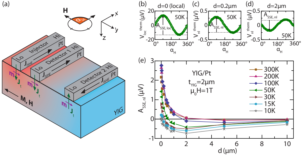
Figure 8.1: (a) Sketch of the YIG/Pt heterostructure: a dc charge current \mathbf{J}_c (not shown here) is applied to the injector strip (left) and the spin Seebeck signal V_{\text{loc}}^{\text{therm}} is detected locally via the ISHE. The corresponding non-local thermal signal V_{\text{nl}}^{\text{therm}} is measured along the detector strips for different strip separations. The color coding gives a qualitative profile of the magnon accumulation \mu_m in the YIG film, where red corresponds to \mu_m < 0 (magnon depletion) and blue to a positive \mu_m (magnon accumulation). In the short distance regime (detector 1), \mu_m < 0 at the injector and detector, such that the same sign is expected for local and non-local SSE. With increasing distance from the injector (detector 2), \mu_m and consequently the spin current across the interface as well as the detected ISHE voltage change sign. (b) Local spin Seebeck voltage in a t_{\text{YIG}} = 2\mu\text{m} thick YIG film detected at the injector strip at 50 K as a function of the in-plane magnetic field orientation \alpha_H with respect to the \mathbf{x} axis. (c), (d) Non-local thermal voltage measured at T = 50\text{ K} at the detector strip for a device with a strip separation of d = 200\text{ nm} and 2\mu\text{m} , respectively. (e) Non-local SSE amplitude A_{\text{SSE,nl}} extracted from in-plane field rotations at temperatures between 10 K and 300 K as a function of the injector-detector separation d . Figure adapted from Ref. [116].
