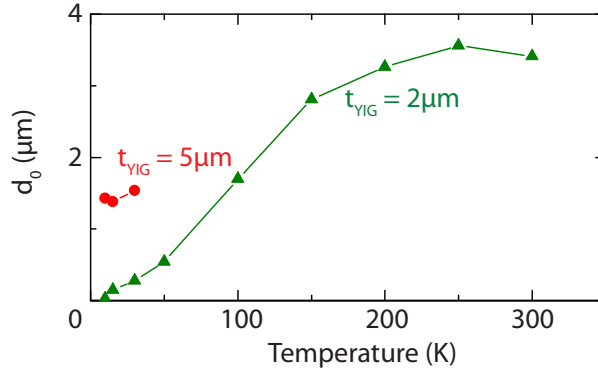
Figure 8.2: Temperature dependence of the critical strip separation d_0 at which the non-local SSE changes sign for the two LPE-YIG films with t_{\text{YIG}} = 5 \mu\text{m} (red dots) and 2 \mu\text{m} (green triangles). Figure adapted from Ref. [116].
