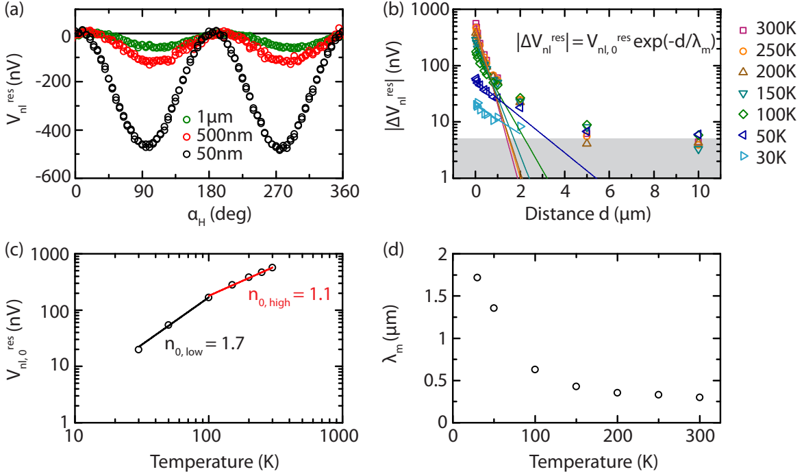
Figure 6.5: (a) V_{nl}^{res} as a function of the ip magnetic field orientation \alpha_H for d = 50 nm, 500 nm and 1 \mu\text{m} at T = 300 K and \mu_0 H = 1 T. (b) V_{nl}^{res} extracted from the ADMR measurements as a function of the strip separation d for different temperatures. The solid lines are fits to the data using Eq. (6.2). (c) V_{nl,0}^{res} - the non-local voltage in the local limit ( d = 0 ) - obtained from the fits in panel (b) as a function of temperature. The solid lines represent power law fits of the form A \cdot T^n . (d) Magnon diffusion length \lambda_m extracted from the exponential decay in panel (b) as a function of temperature.
