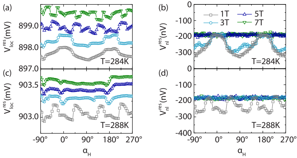
Figure 9.7: Local ADMMR measurement at T = 284\text{ K} (a) and 288\text{ K} (c) for different magnetic fields. V_{\text{loc}}^{\text{res}} no longer follows the typical SMR \cos^2(\alpha_H) dependence, but reveals anisotropic behavior and abrupt jumps when rotating the magnetic field in the sample plane. For better visibility, the curves are offset by a constant value in vertical direction. (b) and (d) Non-local voltage V_{\text{nl}}^{\text{res}} measured in the detector strip: at low magnetic fields the non-local voltage reproduces the same features as the local signal. With increasing field, when no clear angular dependence is discernible in the SMR response, the non-local MMR is constant. This behavior is most likely related to domain formation or anisotropies in the FMI. The remaining negative offset of V_{\text{nl}}^{\text{res}} may be attributed to an electrical cross-talk between the injector and detector strip.
