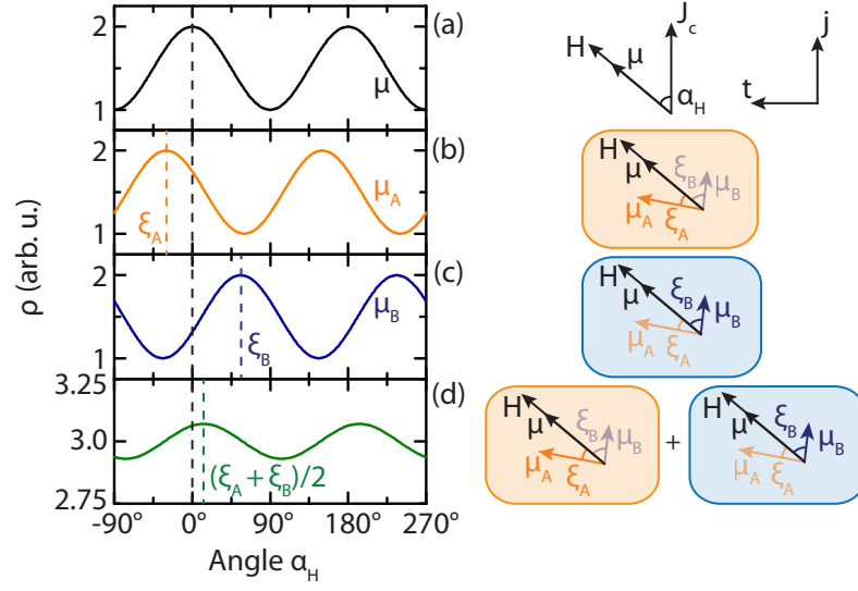
Figure 2.3: Expected SMR response in a two-sublattice FMI/Pt bilayer, where the magnetic moments \mu_A and \mu_B of sublattices A and B are tilted by angles \xi_A and \xi_B with respect to the external magnetic field \mathbf{H} . (a) Angular dependence of the Pt resistivity \rho in the macrospin model: the SMR is governed by the orientation of the net magnetic moment \mu which is aligned with the external magnetic field. The resistivity follows a \cos^2(\alpha_H) dependence where \alpha_H is the angle between the applied magnetic field and the current direction \mathbf{j} . (b) and (c) Expected angular dependence of \rho assuming that only sublattice A or B contribute to the SMR. The \cos^2(\alpha_H) dependence is shifted by the respective canting angle \xi_{A,B} . (d) Total SMR response for equal contributions of both sublattices according to the microscopic model (Eq. (2.14)) with \rho_{1,A} = \rho_{1,B} = \rho_1 . The angular dependence is shifted by a finite angle (\xi_A + \xi_B)/2 compared to the expectations of the macrospin model in panel (a).
