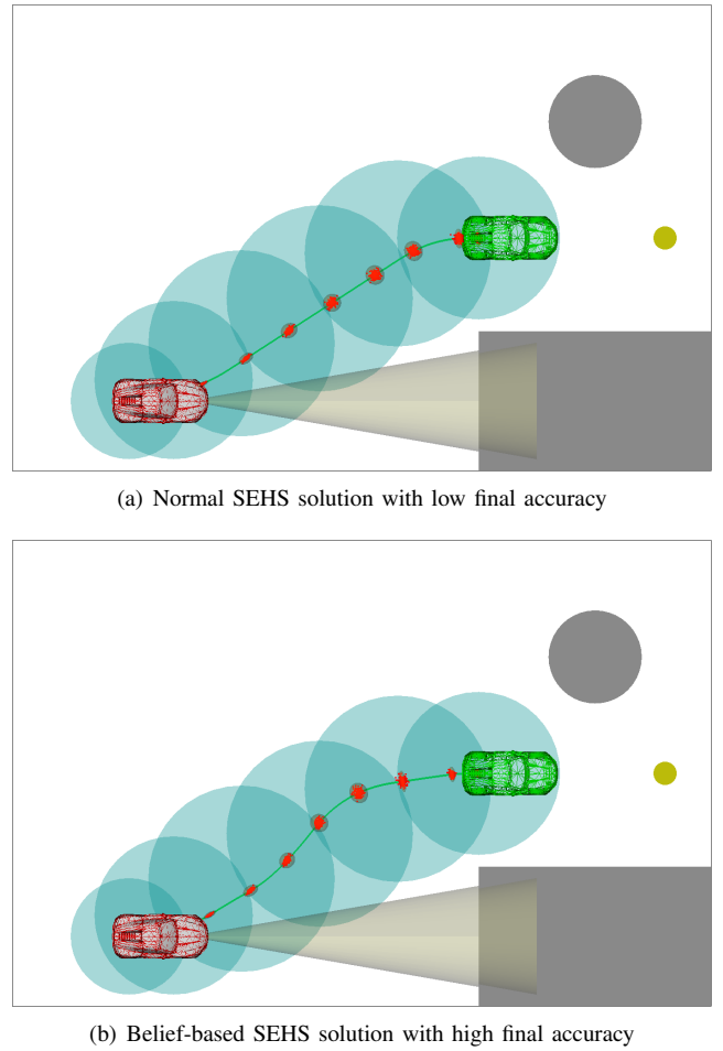
Fig. 5. Precise parking to the goal position with the help of a localization marker (yellow circle). The detection range of the vehicle is illustrated as the light yellow cone.
