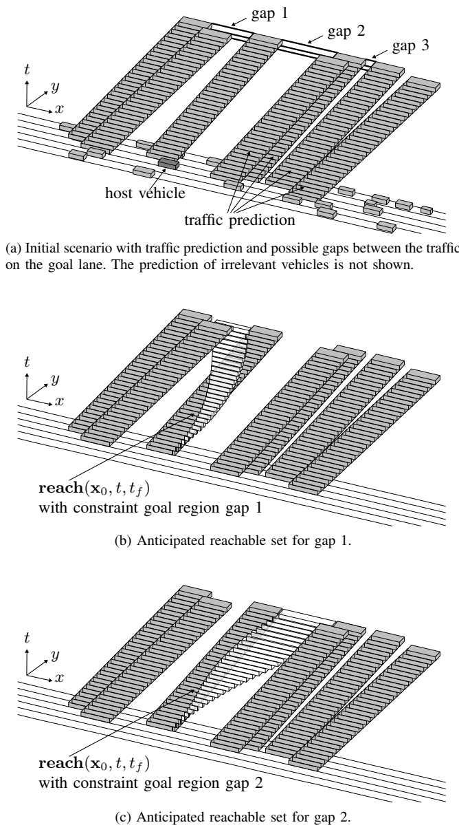
Fig. 7. Lane change scenario with different goal regions.
