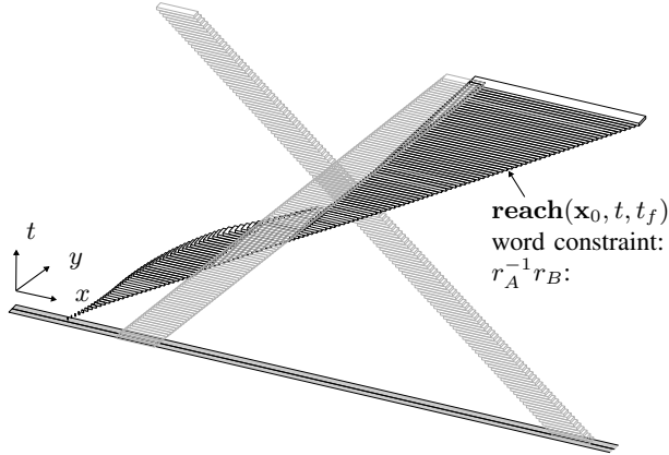
(c) Anticipated reachable set with word constraint r_A^{-1} r_B .
