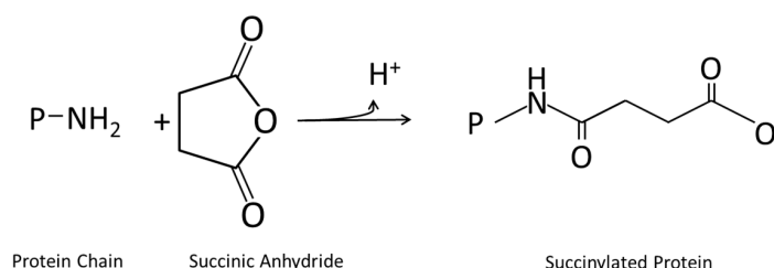
Figure 4. Succinylation of protein chains, adapted from [215].
