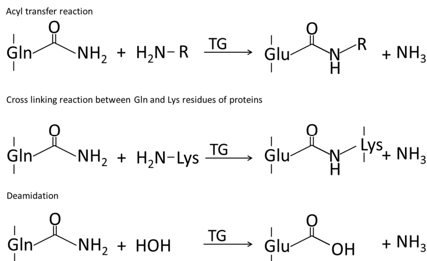
Figure 9. Reactions catalyzed by transglutaminase, adapted from [30].
