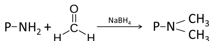
Figure 2. Reductive methylation, adapted from [207].
