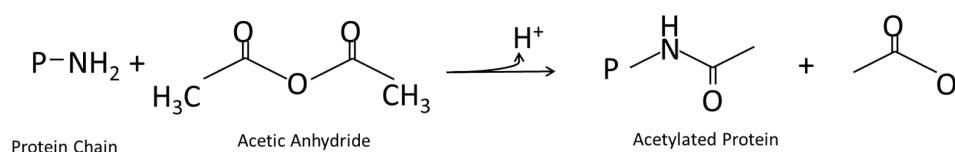
Figure 3. Acetylation of protein chains, adapted from [215].
