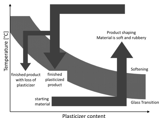
Figure 1. Effect of plasticizer content on thermoplastic processing, adapted from [4].
