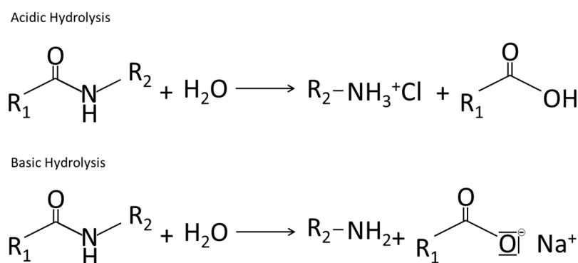
Figure 6. Acidic and Basic Hydrolysis of Proteins, adapted from [30,229].
