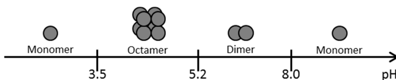
Figure 7. Quaternary structure of \beta -Lg as a function of pH at low temperature and low concentration, adapted from [234].
