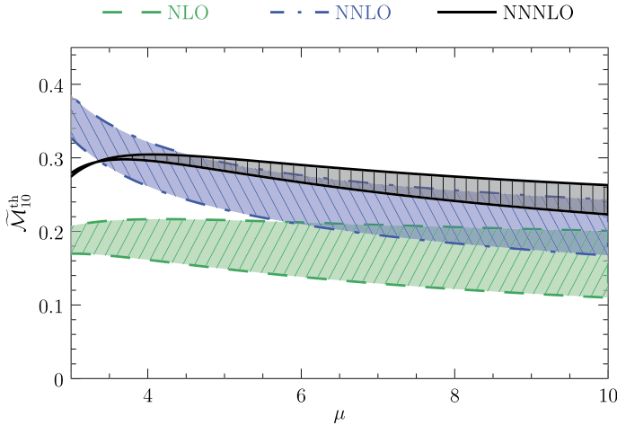
Fig. 3. Scale dependence of \tilde{\mathcal{M}}_{10}^{\text{th}} in (10 \text{ GeV})^{-20} with m_b^{\text{PS}}(2 \text{ GeV}) = 4.5 \text{ GeV} . At each order the shaded band shows the contribution from the continuum cross section. The lower boundary of the band is the moment without the continuum contribution.
