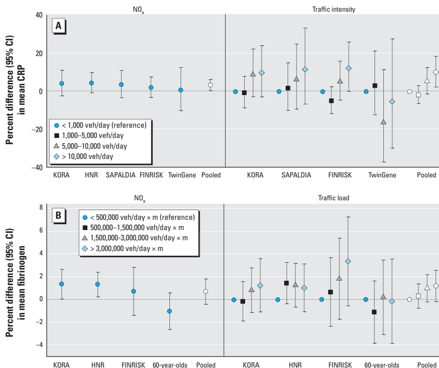
Figure 1. Cohort-specific and pooled effect estimates (the main model) for the associations of NO_x and traffic with inflammatory markers. veh, vehicles. Estimates calculated for a 20\text{-}\mu\text{g}/\text{m}^3 increase in NO_x . (A) NO_x , traffic intensity at the nearest road, and CRP; (B) NO_x , traffic load on major roads within 100 m, and fibrinogen.
