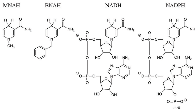
FIGURE 1 | Structural comparison of the biomimetics N -methyl-1,4-dihydropyridin-2(1H)-carboxamide (MNAH) and N -benzyl-1,4-dihydropyridin-2(1H)-carboxamide (BNAH), and the natural cofactors NAD(P)H.
