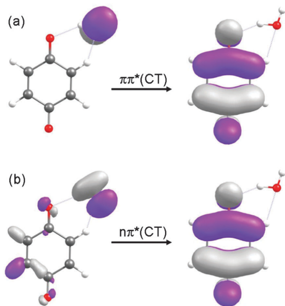
Fig. 4 The molecular orbitals involved in the {}^1\pi\pi^*(CT) and {}^1n\pi^*(CT) states, calculated at R_{O-H} = 1.0 Å, are displayed in (a) and (b), respectively.
