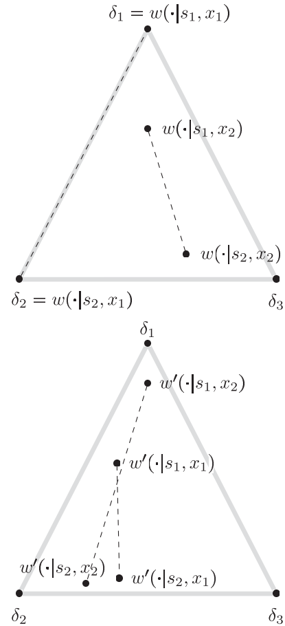
Fig. 3. Light gray lines are the vertices of the probability simplex \mathcal{P}(\{1, 2, 3\}) . The sets \text{conv}(\{w(\cdot|s_1, x_i), w(\cdot|s_2, x_i)\}) where i = 1, 2 are displayed as dashed lines. The intersection of the dashed lines in the lower picture shows that \mathfrak{W}' is symmetrizable.
