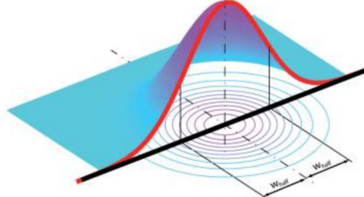
Fig.1: Gauss filter for 2D-filtering (blue surface) and 1D-filtering (red line)
