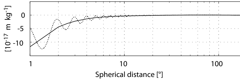
Figure 6: Green's function G(\psi_{PQ}) for the Earth model PREM. Dotted: truncation of the spherical harmonic expansion at degree n = 350 , solid: infinite expansion.
