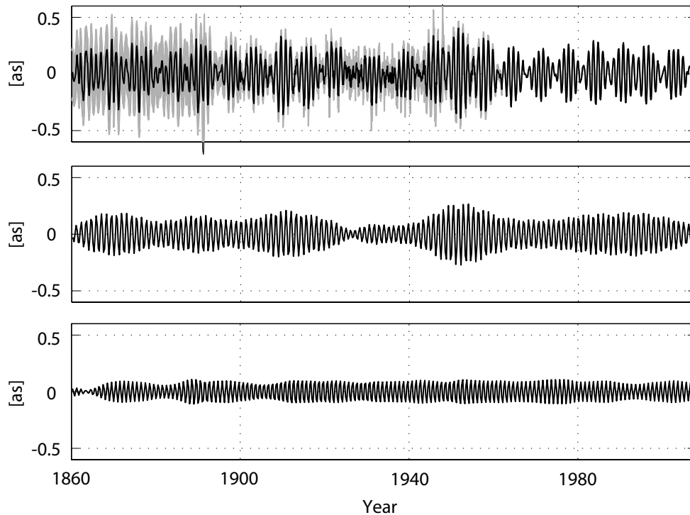
Figure 2: Long-term observations of polar motion ( x -component, linear trend removed) between 1860 and 2009 together with the 3\sigma error margin plotted in grey (top) and Chandler (middle) and annual (bottom) signal component determined by wavelet filtering.
