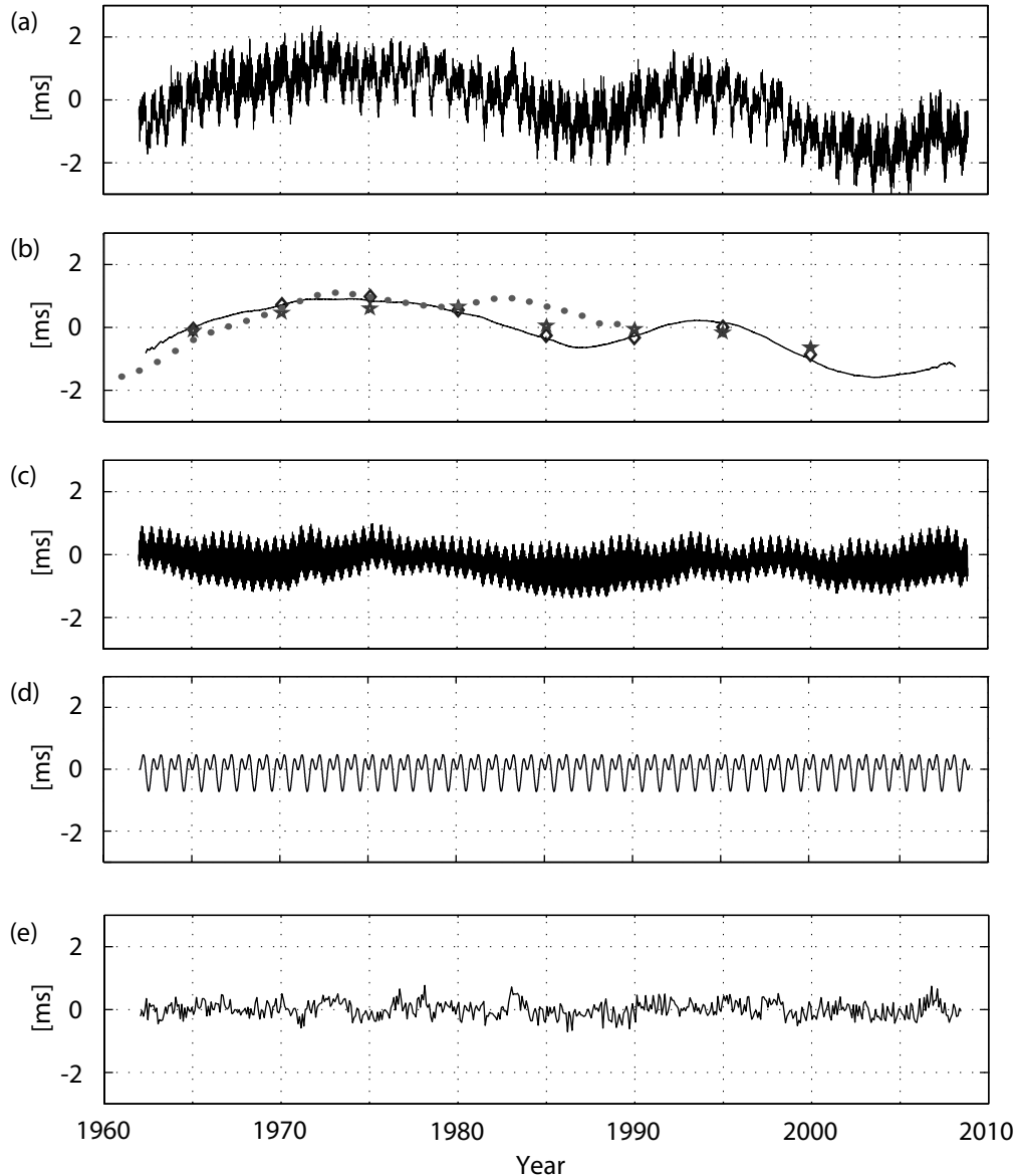
Figure 4: Variations of length-of-day ( \Delta LOD ) for the time frame between 1962 and 2009. (a) Observation time series EOP 05 C04, (b) moving average over five years in comparison with three models for the influence of core-mantle-interaction (dots: JBG; stars: PD1; diamonds: PD2; see text), (c) effect of solid Earth tides, (d) annual and semi-annual signal component, (e) residual time series (a-b-c-d).
