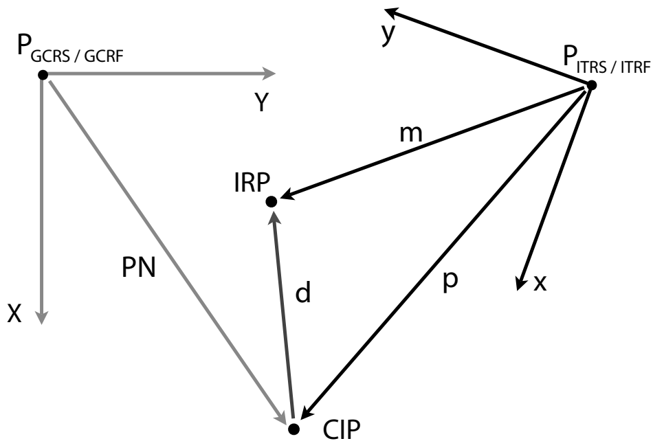
Figure 8: Poles of reference with regard to the coordinate systems ITRS and GCRS (and their respective realisations ITRF/GCRF), and correspondence between model values m(t) and published polar motion values p(t) (MENDES CERVEIRA et al. 2009).
