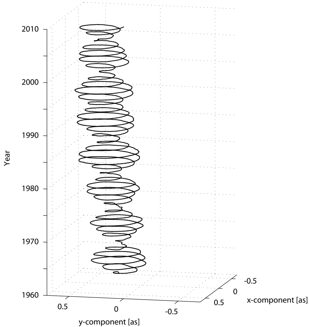
Figure 1: Observations of polar motion from the EOP 05 C04 series of the IERS between 1962 and 2009.
