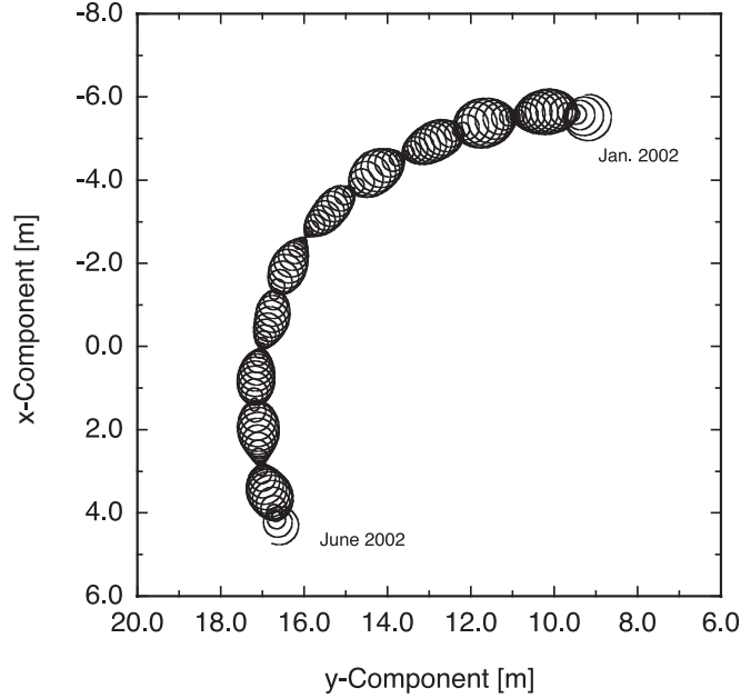
Figure 3: Path of the rotation pole in the Earth-fixed reference system between January and June 2002 in metres on the Earth surface (Figure taken from SCHREIBER et al. 2004).
