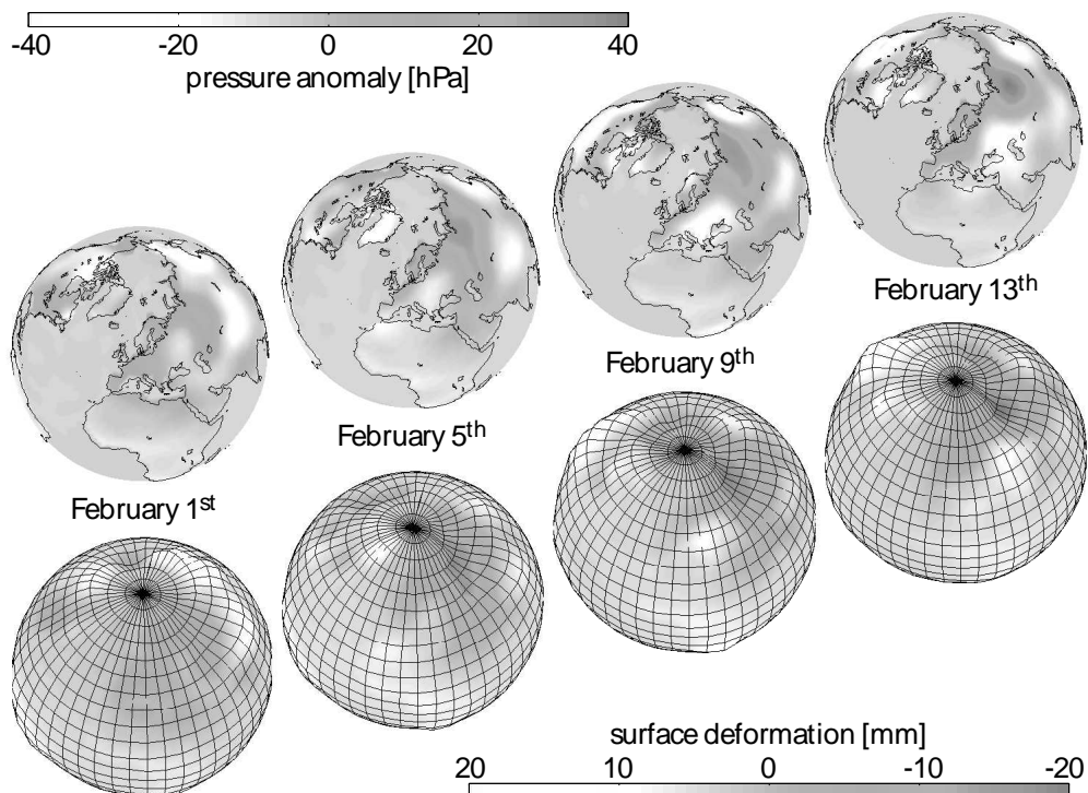
Figure 7: Deformations of the solid Earth due to anomalies of atmospheric surface pressure, ocean bottom pressure, and continental water storage (SEITZ 2004).
