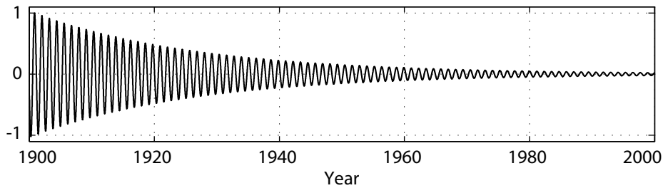
Figure 5: Damped Chandler oscillation ( x -component) derived from a simulation study with a dynamic Earth system model over 100 years regarding ocean pole tides and mantle anelasticity (SEITZ et al. 2004).
