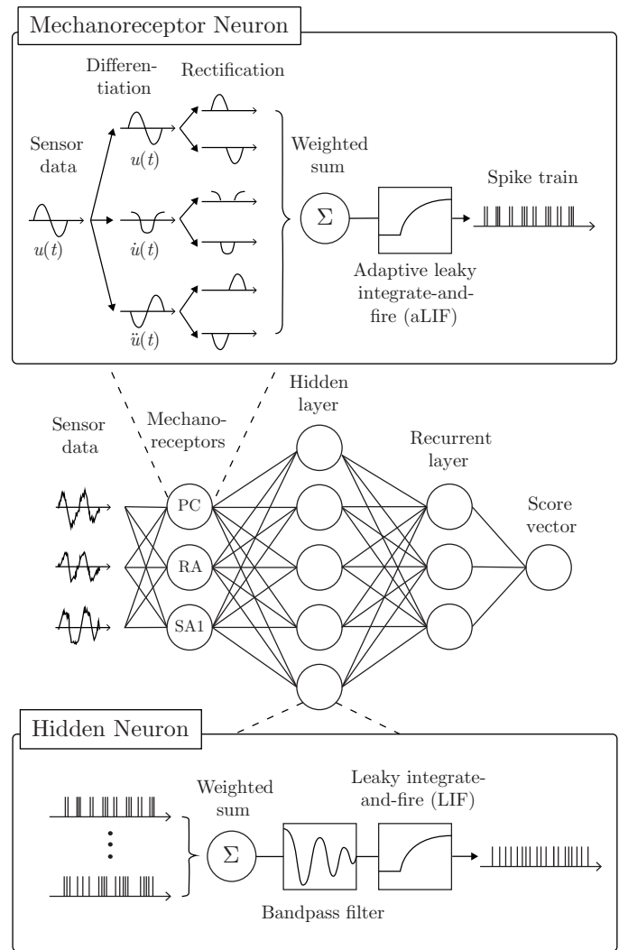
Fig. 1. Architecture of the surface texture classifier. Data from three sensors are encoded in the spiking activity of mechanoreceptor neurons. A hidden layer extracts nonlinear features of these spike trains in the frequency domain by convolution with bandpass filters. A recurrently connected output (feedback arrows omitted) represents the score for each class, smoothed over time. This score vector is linearly decoded from the recurrent layer to find the texture with the largest score. Connection weights and neural parameters are given by the principles of the NEF.
