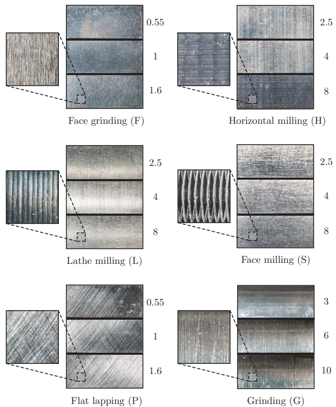
Fig. 3. Detailed photographs of surface textures used to test the system. This set was manufactured using 6 different metal surface finishing methods, with 3 roughnesses per finishing method, for a total of 18 distinct textures. The mean roughness depth (Rz) is indicated to the right of each texture.
