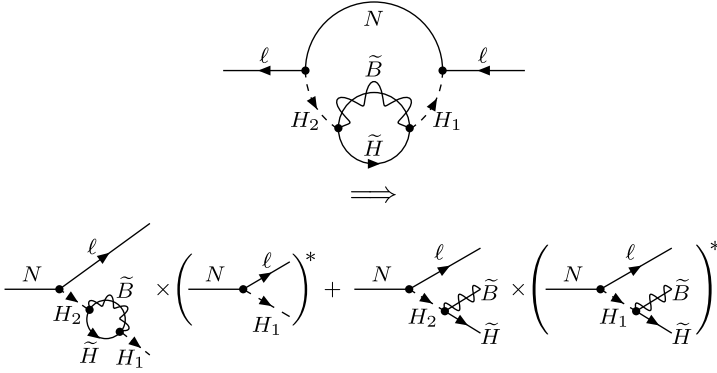
Fig. 7. Diagrams that lead to potential contributions to the lepton asymmetry but that are vanishing when H , \tilde{H} and \tilde{B} are in equilibrium. In the interference terms, we have suppressed the notation of the integrals over the phase space of the external particles other than \ell . Notice that when H_1 corresponds to a RIS, the 1 \leftrightarrow 3 amplitudes can be cut along H_1 and fused along \tilde{B} and \tilde{H} , such that they cancel the interference of the 1 \leftrightarrow 2 amplitudes, as it is explained in Section 5.
