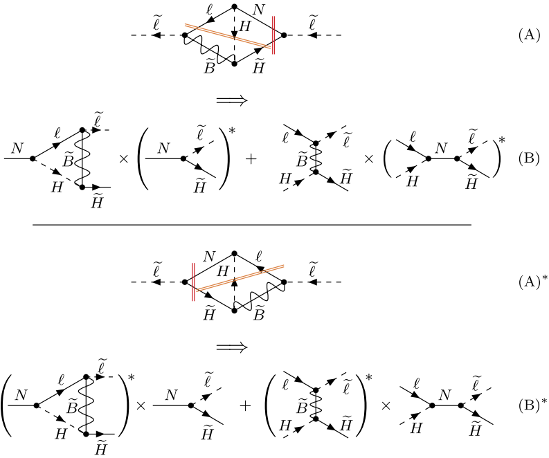
Fig. 4. Relation of the slepton CTP self-energies (A), (A)* to the CPV interference of amplitudes (B), (B)* in conventional approaches, on the example of the contribution from the off-shell \tilde{B} , where the star indicates that the diagrams represent terms that are related by complex conjugation. The CPV contributions to the interference terms occur when \ell and H are on-shell. The RIS contribution arises from an on-shell N in the 2 \leftrightarrow 2 scattering amplitude. In the interference terms, we have suppressed the notation of the integration over the phase space of the external particles other than \tilde{\ell} .
