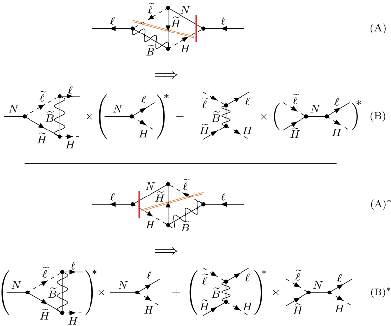
Fig. 3. Relation of the lepton CTP self-energies (A), (A)* to the CPV interference of amplitudes (B), (B)* in conventional approaches, on the example of the contribution from the off-shell \tilde{B} , where the star indicates that the diagrams represent terms that are related by complex conjugation. The CPV contributions to the interference terms occur when \tilde{\ell} and \tilde{H} are on-shell. The RIS contribution arises from an on-shell N in the 2 \leftrightarrow 2 scattering amplitude. In the interference terms, we have suppressed the notation of the integration over the phase space of the external particles other than \ell .
