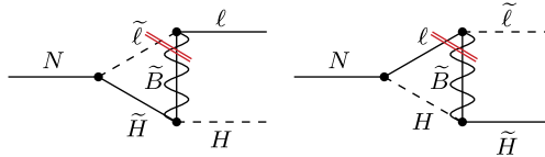
Fig. 5. Cuts in vacuum diagrams with off-shell Higgsino and Higgs boson.
