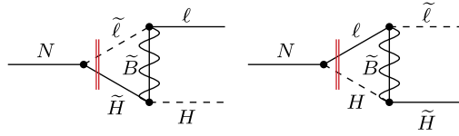
Fig. 2. Cuts in vacuum diagrams with off-shell bino.
