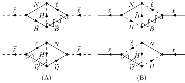
Fig. 1. The vertex-type self-energies i\Pi_{\tilde{\ell}}^y (A) and i\Sigma_{\ell}^y (B).
