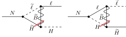
Fig. 6. Cuts in vacuum diagrams with off-shell slepton and lepton.
