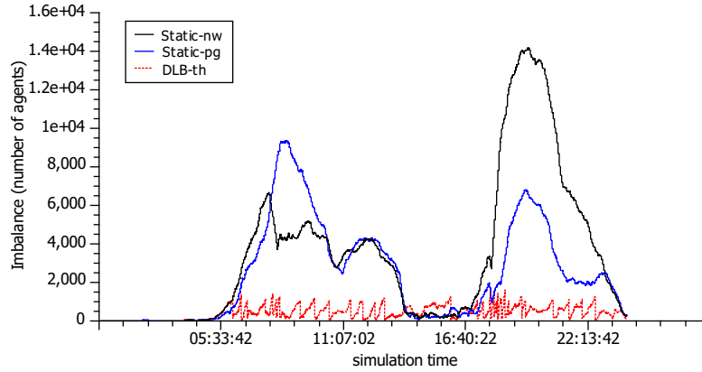
Figure 3: Comparison of workload imbalance of 4 processes throughout the simulation.
