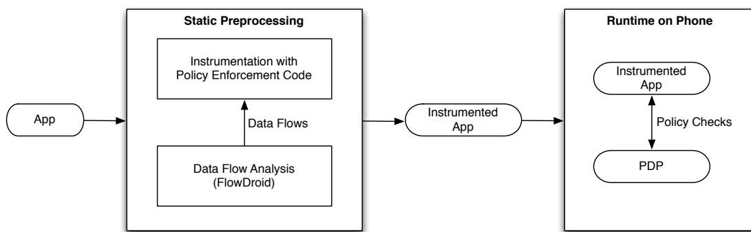
Fig. 1. DROIDFORCE Architecture Overview
