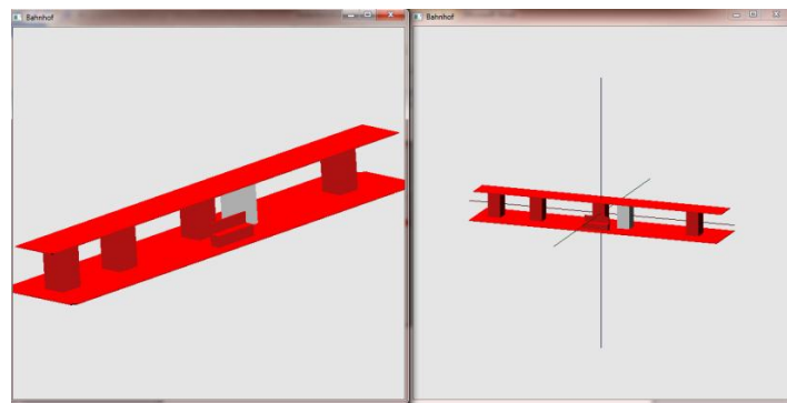
Figure 8: Synchronous working: Client 2 (right) immediately sees the modified position of the pillar.
