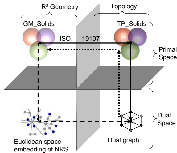
Fig. 4.5 Sensor space
