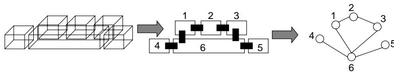
Fig. 4.3 Example for the partitioning of building interior into rooms and its representation in dual space
