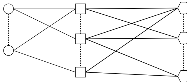
Fig. 4.7 Example for a tripartite graph containing nodes from three layers. Nodes of different layers are connected by joint-state edges. Only one state in each partition can be active and active states must be connected to each other by joint-state edges. The dashed edges represent cell adjacencies within each layer.
