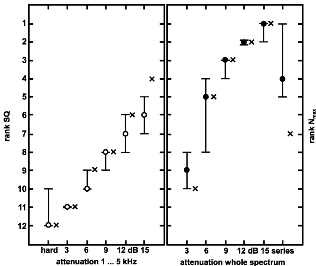
Figure 19: Improvement of the sound quality of a Diesel motor with “hard” motor adjustment when adding simulated absorptive measures. Circles: subjective sound quality estimates, crosses: physical measurements of loudness (after Patsouras et al. 2001)
