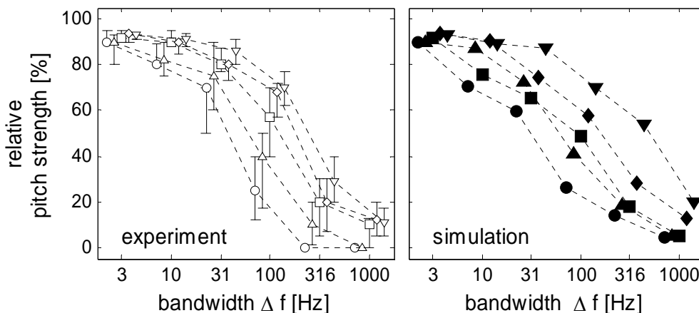
Figure 11: Pitch strength of narrow-band noises as a function of bandwidth. Subjective evaluations (Wiesmann and Fastl 1991, left panel) and predictions by the model of pitch strength (Fruhmann 2006a, right panel)
