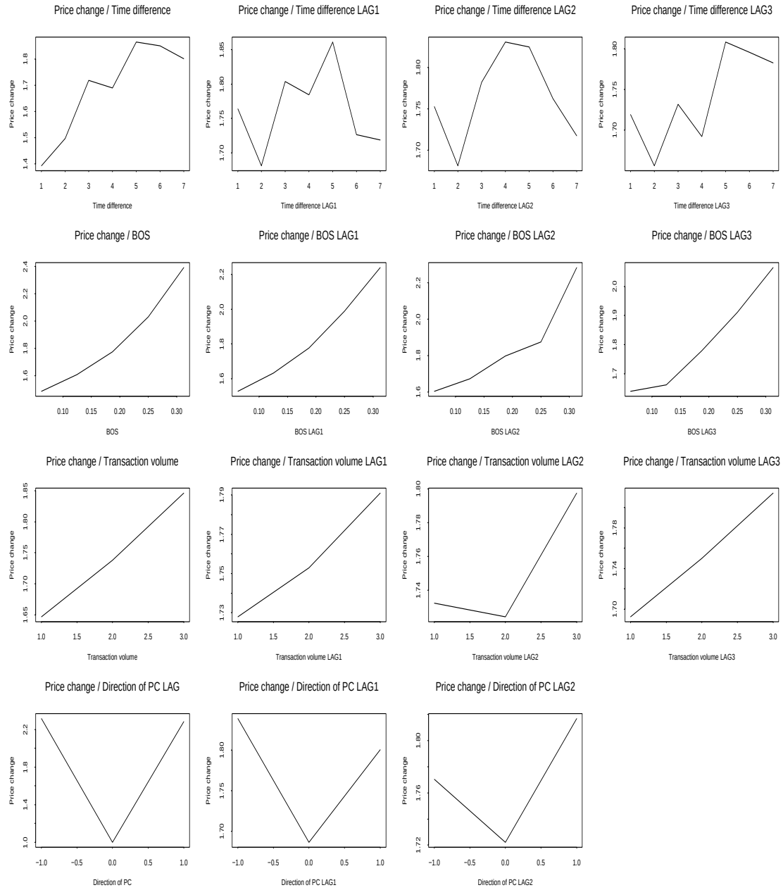
Figure 1: Observed relationships between average PC values per category and different levels of the covariates TD, SIZE, BOS, and DIR.
