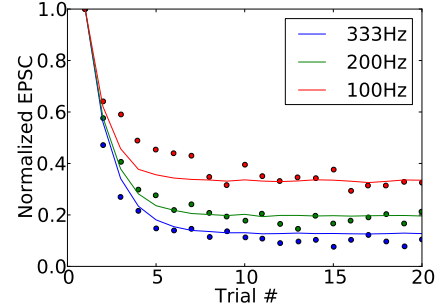
Figure 1: Relative postsynaptic currents in response to electrical shocks to the ANF at three different frequencies. Dots represent experimental data from [4] (Fig. 2d), lines show the best fit to the model.
