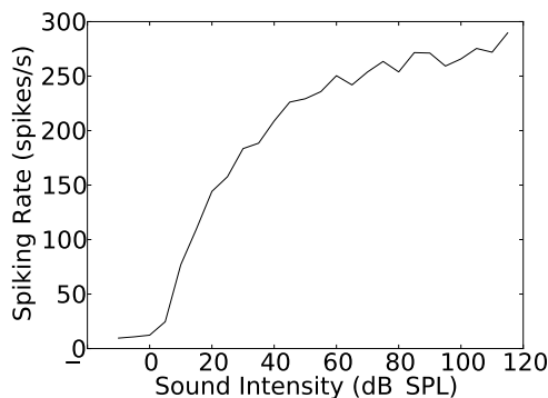
Figure 4: Rate-intensity characteristic of a simulated GBC. Spontaneous and saturation rates are correct. However dynamic range in real neurons is usually smaller than 35 dB.
