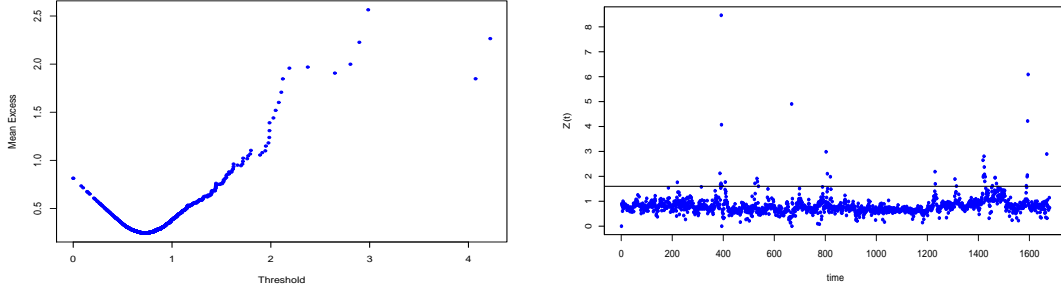
FIGURE 7. Left: ME plot of Z(\cdot) , right: Z(\cdot) with chosen threshold u = 1.62 .
