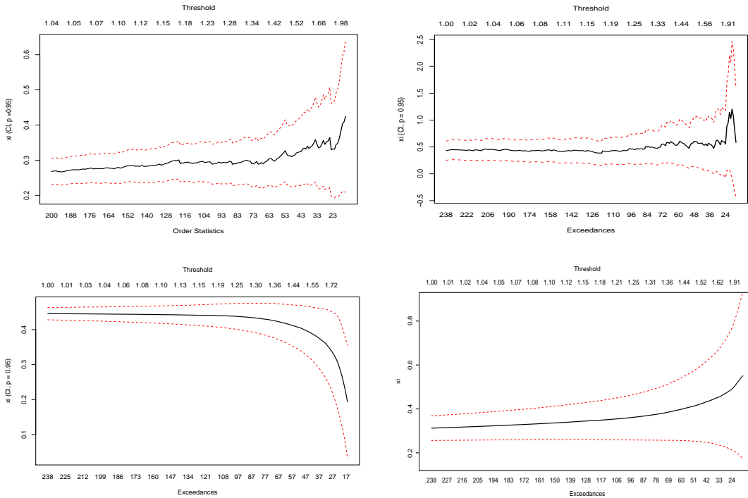
FIGURE 8. Different estimates of \xi for different thresholds with asymptotic 95% point-wise confidence bands: left: \hat{\xi}_{Hill} , right: \hat{\xi}_{MLE} , lower left: \hat{\xi}_{ME} , lower right: \hat{\xi}_{QQ} .
