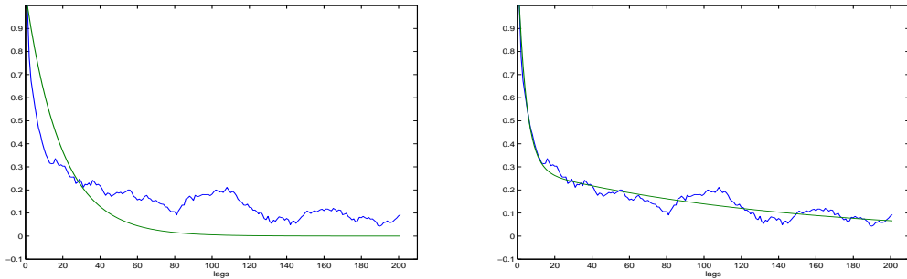
FIGURE 11. Left: Fit of the estimated autocorrelation function of X_2 with one factor. Right: Fit with two factors.
