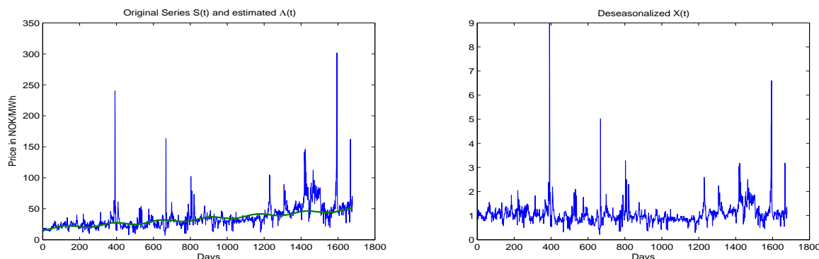
FIGURE 6. Left: Original series S(\cdot) and estimated \widehat{\Lambda}(\cdot) . Right: Deseasonalized series X(\cdot) .
