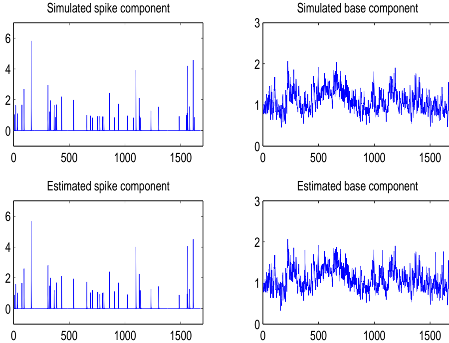
FIGURE 14. The true (top) in comparison with estimated (bottom) spike and base component for one simulated spot price path.
