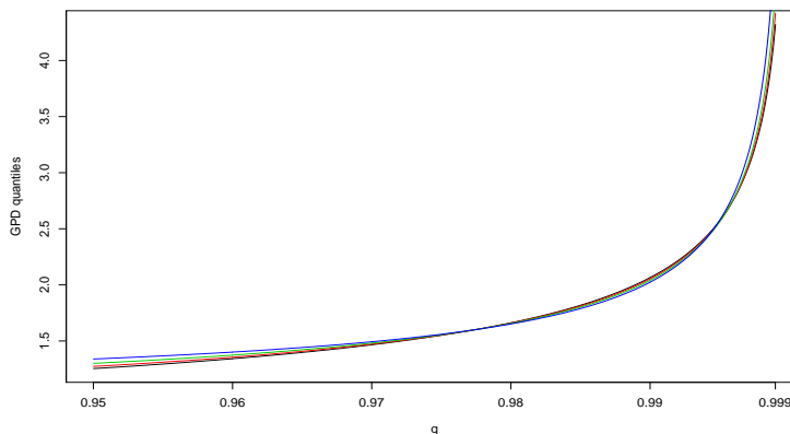
FIGURE 9. Four different estimates of the quantile function in the relevant risk management area based on the above different estimates for \xi and \beta for threshold u = 1.62 .
