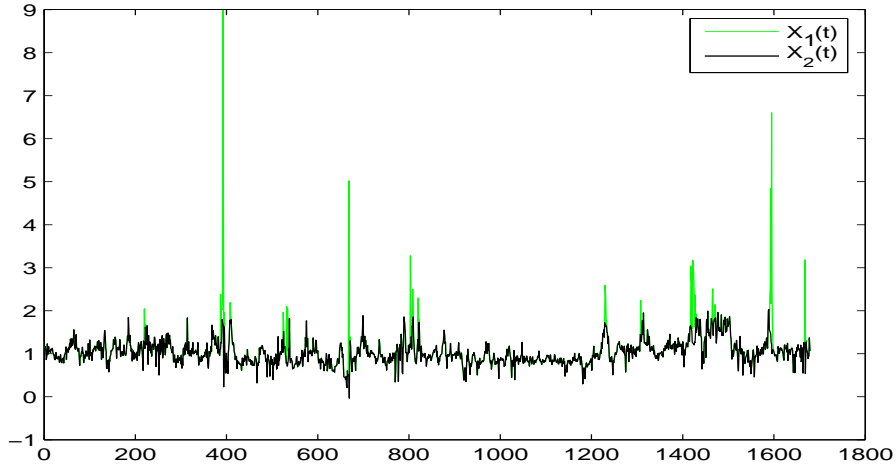
FIGURE 10. Decomposition of X(\cdot) into the spike component X_1(\cdot) and the base component X_2(\cdot) .
