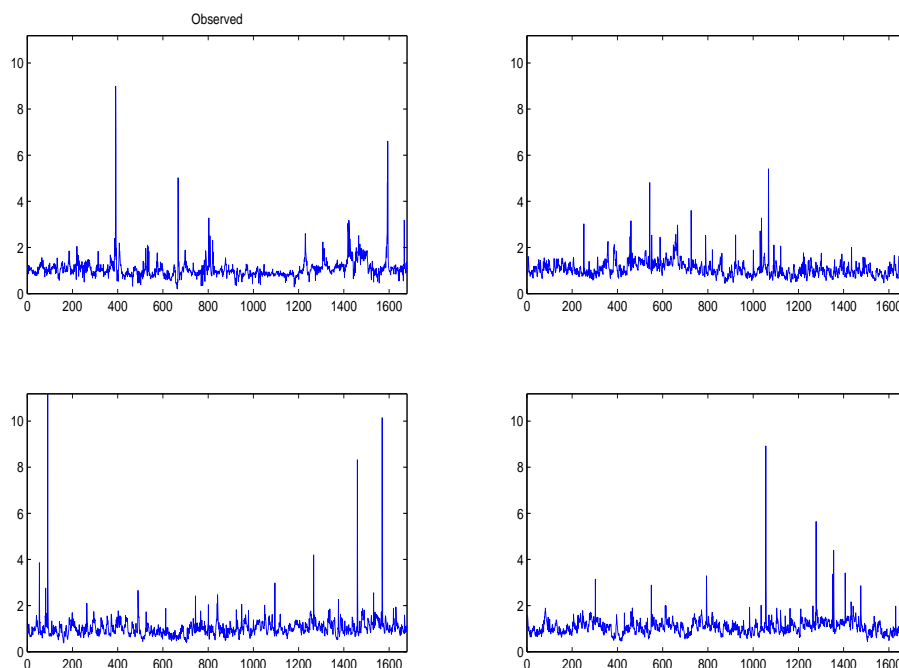
FIGURE 13. Three simulated paths in comparison with the data X(\cdot) (top left)
