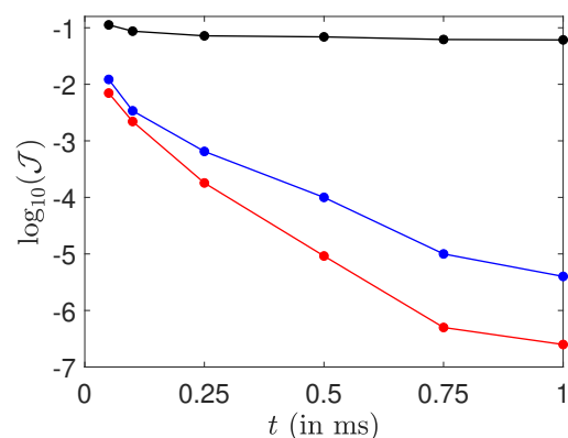
Figure 5. Evolution of the logarithm of the cost functional \mathcal{J} as a function of the control time for different maximum amplitudes (black, 30 \text{ V}\cdot\text{m}^{-1} ; blue or dark gray, 50 \text{ V}\cdot\text{m}^{-1} ; red or light gray, 70 \text{ V}\cdot\text{m}^{-1} ).
