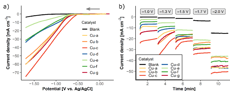
Figure 3. (a) LSV and (b) CA measurements of the synthesized copper catalysts in \text{CO}_2 -saturated 0.5 M \text{KHCO}_3 , blank = carbon paper without catalyst. LSV was measured from open circuit potential (OCP) to -1.7 V vs. Ag/AgCl. CA measurements were performed at the different step potentials -1.0 , -1.3 , -1.5 , -1.7 , and -2.0 V vs. Ag/AgCl for 2 min each.
