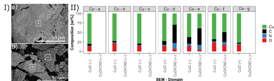
Figure 1. (I) SEM images of (a) Cu-b and (b) Cu-f. (II) Elemental composition (EDX) of synthesized copper catalysts Cu-a, Cu-b, Cu-c, Cu-d, Cu-e, Cu-f, and Cu-g.
