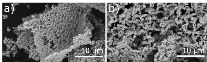
Figure 2. SEM images of (a) Cu-a and (b) Cu-c. Cu-a shows a frilled and compact CuO structure obtained from CuNP precursor, and Cu-c shows large pores and a less dense ordered structure from CuO as precursor.
