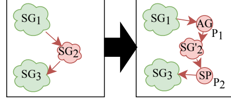
(a) Early-Aggregation
