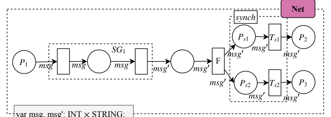
(b) After applying the rewrite rule
