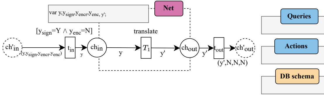
Figure 19: Example: message translator construction
