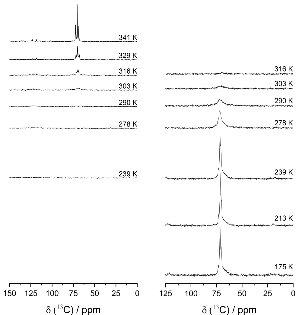
Figure 6. Temperature-dependent ^{13}\text{C} -MAS spectra (left) and ^{13}\text{C} - \{^1\text{H}\} -CP-MAS spectra (right) for the PEO: \text{Mg}(\text{TFSI})_2 36:1 membrane for the indicated temperatures.
